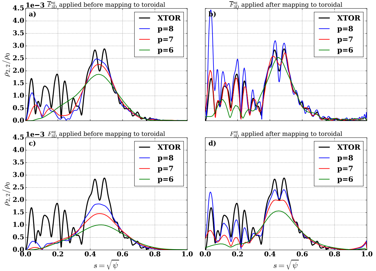
Figure 10. Radial structure of the m = 2, n = 2 mode. Filtering before the mapping and with \bar{F}_{3D}^{sg} (a), after the mapping and with \bar{F}_{3D}^{sg} (b), before the mapping and with F_{3D}^{sg} (c), after the mapping and with F_{3D}^{sg} (d).
