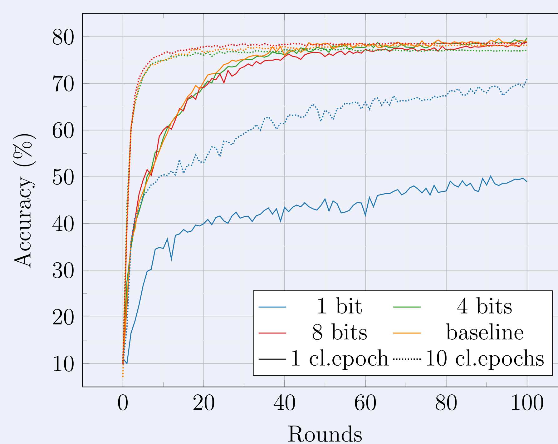
Accuracy evolution comparison, for the quantization technique, between baseline (FP 32-bit), 1-bit, 4-bit and 8-bit, on the left. Pruning effect on the accuracy in function of the pruning rate, where the rate indicates the % of total parameters pruned, on the right. Experiments done for 1 and 10 cl.epochs (clients epochs)
