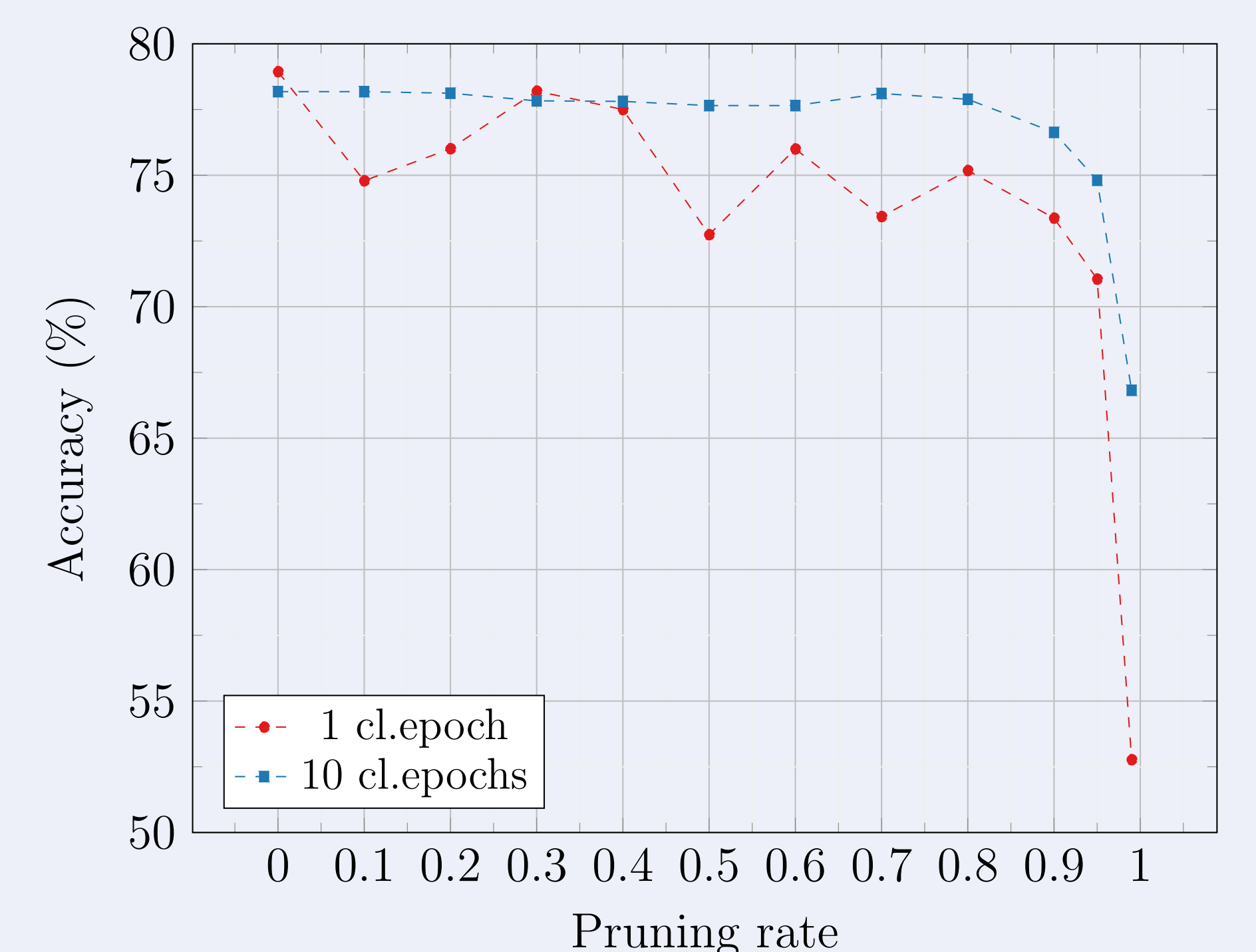
Accuracy evolution comparison, for the quantization technique, between baseline (FP 32-bit), 1-bit, 4-bit and 8-bit, on the left. Pruning effect on the accuracy in function of the pruning rate, where the rate indicates the % of total parameters pruned, on the right. Experiments done for 1 and 10 cl.epochs (clients epochs)
