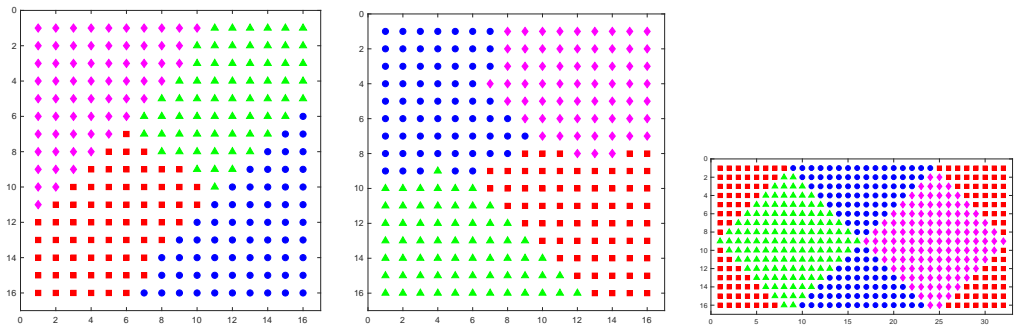
(a) The K = 4 -way partition of the 16 \times 16 obtained by the special routines [26]. Connectivity-1 is 58.
