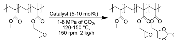
Scheme 6 Carbonatation of Lotader® AX8900 in an extruder.
