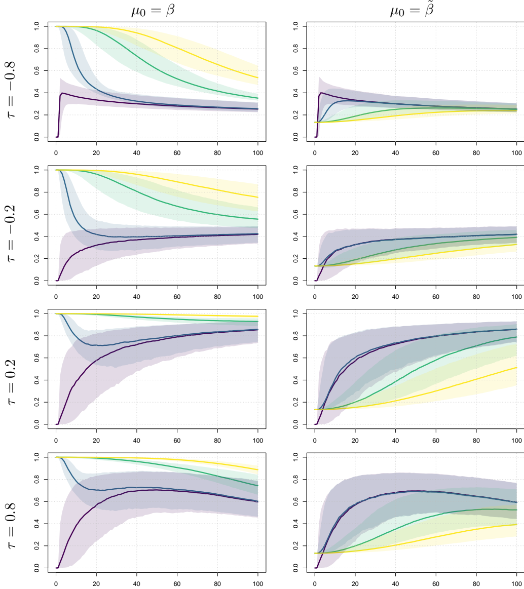
Figure 7: Finite sample behavior of the SEPALS estimator computed with the conjugate prior on simulated data in dimension d = 30 from a Pareto distribution ( \gamma_Y = 1/5 , a = 2 ) and a (rotated) Clayton copula with Kendall's tau \tau \in \{-0.8, -0.2, 0.2, 0.8\} (from top to bottom). The power of the link function g(t) = t^c is fixed to c = 1/4 . Vertically: R(Y_{n-k+1,n}) between \hat{\beta}_{\text{map}}^c and \beta for a prior direction \mu_0 = \beta (left) or \mu_0 = \tilde{\beta} (right) as a function of the number k \in \{1, \dots, 100\} of exceedances (horizontally). The concentration parameter is \kappa_0 \in \{0, 10^{-4}, 3 \cdot 10^{-3}, 10^{-2}\} , respectively in violet, blue, green and yellow. Coloured areas correspond to 90% confidence intervals.
