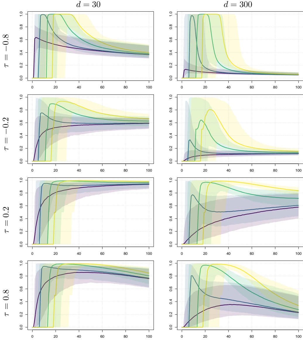
Figure 8: Finite sample behavior of the SEPALS estimator computed with the sparse prior on simulated data in dimension d = 30 (left) and d = 300 (right) from a Pareto distribution ( \gamma_Y = 1/5 , a = 2 ) and a (rotated) Clayton copula with Kendall's tau \tau \in \{-0.8, -0.2, 0.2, 0.8\} (from top to bottom). The power of the link function g(t) = t^c is fixed to c = 1 . Vertically: R(Y_{n-k+1,n}) between \hat{\beta}_{\text{map}}^s and \beta for as a function of the number k \in \{1, \dots, 100\} of exceedances (horizontally). The concentration parameter is \lambda \in \{0, 10^{-4}, 5 \cdot 10^{-4}, 10^{-3}\} , respectively in violet, blue, green and yellow. Coloured areas correspond to 90% confidence intervals.
