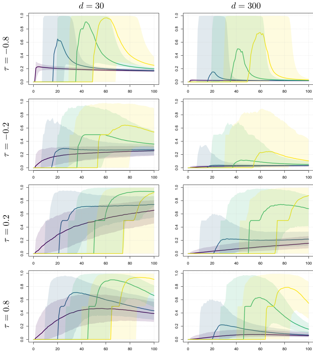
Figure 10: Finite sample behavior of the SEPALS estimator computed with the sparse prior on simulated data in dimension d = 30 (left) and d = 300 (right) from a Pareto distribution ( \gamma_Y = 1/5 , a = 2 ) and a (rotated) Clayton copula with Kendall's tau \tau \in \{-0.8, -0.2, 0.2, 0.8\} (from top to bottom). The power of the link function g(t) = t^c is fixed to c = 1/4 . Vertically: R(Y_{n-k+1,n}) between \hat{\beta}_{\text{map}}^s and \beta for as a function of the number k \in \{1, \dots, 100\} of exceedances (horizontally). The concentration parameter is \lambda \in \{0, 10^{-4}, 5 \cdot 10^{-4}, 10^{-3}\} , respectively in violet, blue, green and yellow. Coloured areas correspond to 90% confidence intervals.
