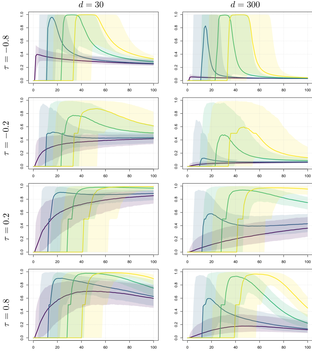
Figure 9: Finite sample behavior of the SEPALS estimator computed with the sparse prior on simulated data in dimension d = 30 (left) and d = 300 (right) from a Pareto distribution ( \gamma_Y = 1/5 , a = 2 ) and a (rotated) Clayton copula with Kendall's tau \tau \in \{-0.8, -0.2, 0.2, 0.8\} (from top to bottom). The power of the link function g(t) = t^c is fixed to c = 1/2 . Vertically: R(Y_{n-k+1,n}) between \hat{\beta}_{\text{map}}^s and \beta for as a function of the number k \in \{1, \dots, 100\} of exceedances (horizontally). The concentration parameter is \lambda \in \{0, 10^{-4}, 5 \cdot 10^{-4}, 10^{-3}\} , respectively in violet, blue, green and yellow. Coloured areas correspond to 90% confidence intervals.
