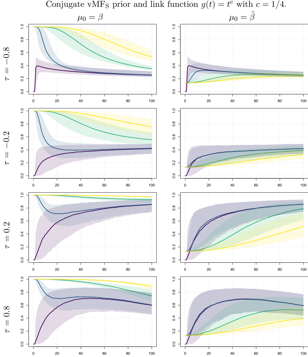
Figure 7: Finite sample behavior of the SEPALS estimator computed with the conjugate prior on simulated data in dimension d = 30 from a Pareto distribution ( \gamma_Y = 1/5 , a = 2 ) and a (rotated) Clayton copula with Kendall's tau \tau \in \{-0.8, -0.2, 0.2, 0.8\} (from top to bottom). The power of the link function g(t) = t^c is fixed to c = 1/4 . Vertically: R(Y_{n-k+1,n}) between \hat{\beta}_{\text{map}}^c and \beta for a prior direction \mu_0 = \beta (left) or \mu_0 = \tilde{\beta} (right) as a function of the number k \in \{1, \dots, 100\} of exceedances (horizontally). The concentration parameter is \kappa_0 \in \{0, 10^{-4}, 3 \cdot 10^{-3}, 10^{-2}\} , respectively in violet, blue, green and yellow. Coloured areas correspond to 90% confidence intervals.
