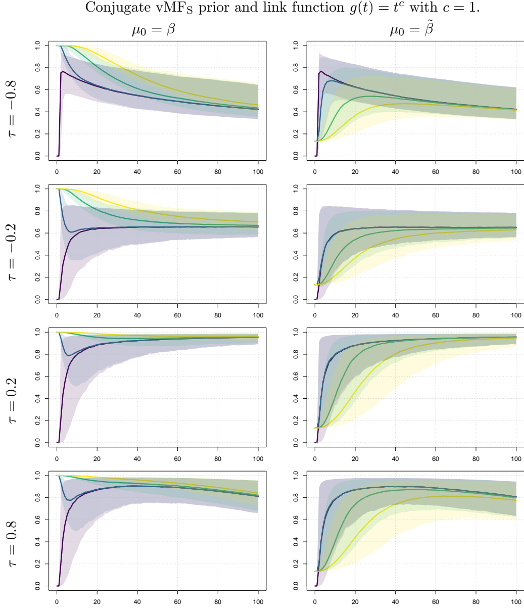
Figure 3: Finite sample behavior of the SEPALS estimator computed with the conjugate prior on simulated data in dimension d = 30 from a Pareto distribution ( \gamma_Y = 1/5 , a = 2 ) and a (rotated) Clayton copula with Kendall's tau \tau \in \{-0.8, -0.2, 0.2, 0.8\} (from top to bottom). The power of the link function g(t) = t^c is fixed to c = 1 . Vertically: R(Y_{n-k+1,n}) between \hat{\beta}_{\text{map}}^c and \beta for a prior direction \mu_0 = \beta (left) or \mu_0 = \tilde{\beta} (right) as a function of the number k \in \{1, \dots, 100\} of exceedances (horizontally). The concentration parameter is \kappa_0 \in \{0, 10^{-4}, 3 \cdot 10^{-3}, 10^{-2}\} , respectively in violet, blue, green and yellow. Coloured areas correspond to 90% confidence intervals.
