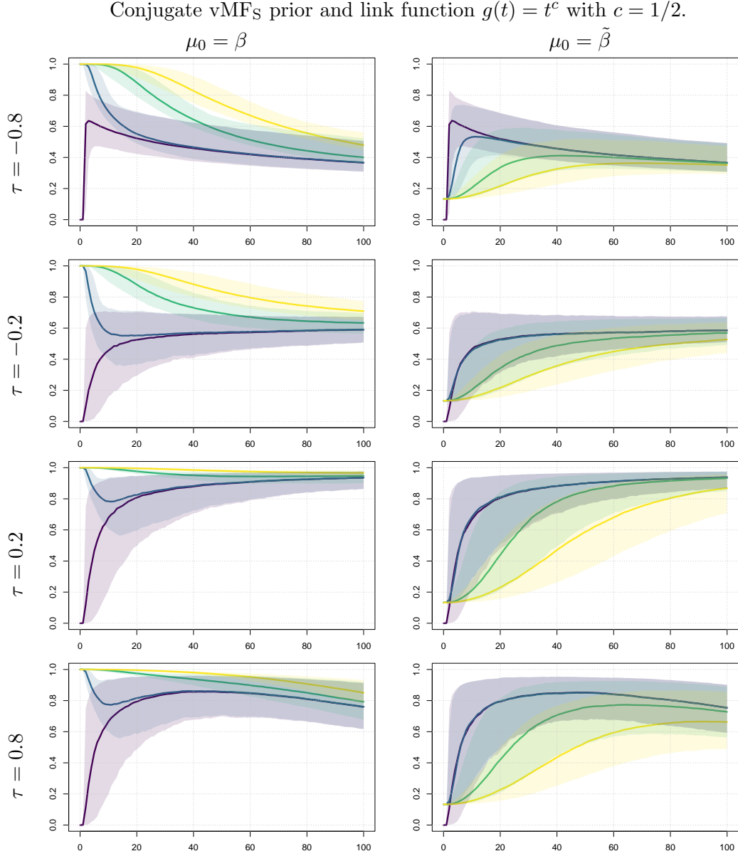
Figure 6: Finite sample behavior of the SEPALS estimator computed with the conjugate prior on simulated data in dimension d = 30 from a Pareto distribution ( \gamma_Y = 1/5 , a = 2 ) and a (rotated) Clayton copula with Kendall's tau \tau \in \{-0.8, -0.2, 0.2, 0.8\} (from top to bottom). The power of the link function g(t) = t^c is fixed to c = 1/2 . Vertically: R(Y_{n-k+1,n}) between \hat{\beta}_{\text{map}}^c and \beta for a prior direction \mu_0 = \beta (left) or \mu_0 = \tilde{\beta} (right) as a function of the number k \in \{1, \dots, 100\} of exceedances (horizontally). The concentration parameter is \kappa_0 \in \{0, 10^{-4}, 3 \cdot 10^{-3}, 10^{-2}\} , respectively in violet, blue, green and yellow. Coloured areas correspond to 90% confidence intervals.
