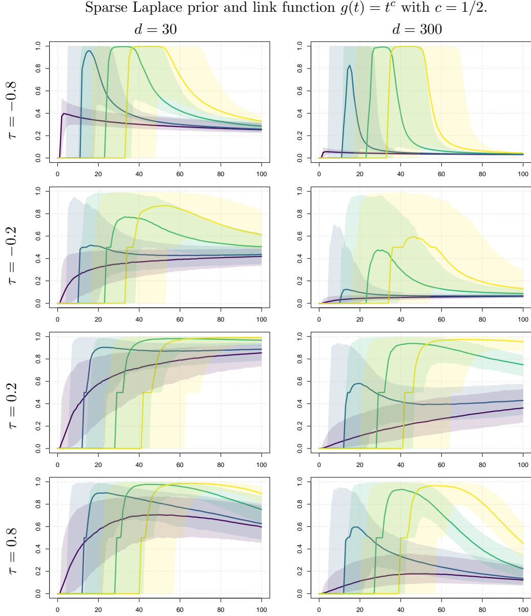
Figure 9: Finite sample behavior of the SEPALS estimator computed with the sparse prior on simulated data in dimension d = 30 (left) and d = 300 (right) from a Pareto distribution ( \gamma_Y = 1/5 , a = 2 ) and a (rotated) Clayton copula with Kendall's tau \tau \in \{-0.8, -0.2, 0.2, 0.8\} (from top to bottom). The power of the link function g(t) = t^c is fixed to c = 1/2 . Vertically: R(Y_{n-k+1,n}) between \hat{\beta}_{\text{map}}^s and \beta for as a function of the number k \in \{1, \dots, 100\} of exceedances (horizontally). The concentration parameter is \lambda \in \{0, 10^{-4}, 5 \cdot 10^{-4}, 10^{-3}\} , respectively in violet, blue, green and yellow. Coloured areas correspond to 90% confidence intervals.
