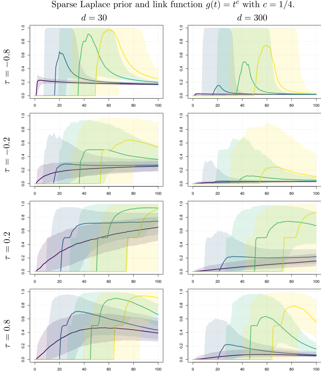
Figure 10: Finite sample behavior of the SEPALS estimator computed with the sparse prior on simulated data in dimension d = 30 (left) and d = 300 (right) from a Pareto distribution ( \gamma_Y = 1/5 , a = 2 ) and a (rotated) Clayton copula with Kendall's tau \tau \in \{-0.8, -0.2, 0.2, 0.8\} (from top to bottom). The power of the link function g(t) = t^c is fixed to c = 1/4 . Vertically: R(Y_{n-k+1,n}) between \hat{\beta}_{\text{map}}^s and \beta for as a function of the number k \in \{1, \dots, 100\} of exceedances (horizontally). The concentration parameter is \lambda \in \{0, 10^{-4}, 5 \cdot 10^{-4}, 10^{-3}\} , respectively in violet, blue, green and yellow. Coloured areas correspond to 90% confidence intervals.
