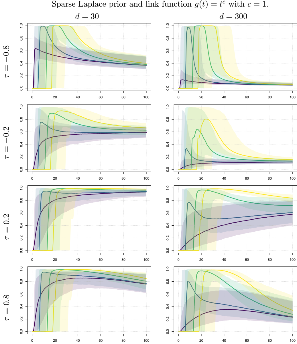
Figure 8: Finite sample behavior of the SEPALS estimator computed with the sparse prior on simulated data in dimension d = 30 (left) and d = 300 (right) from a Pareto distribution ( \gamma_Y = 1/5 , a = 2 ) and a (rotated) Clayton copula with Kendall's tau \tau \in \{-0.8, -0.2, 0.2, 0.8\} (from top to bottom). The power of the link function g(t) = t^c is fixed to c = 1 . Vertically: R(Y_{n-k+1,n}) between \hat{\beta}_{\text{map}}^s and \beta for as a function of the number k \in \{1, \dots, 100\} of exceedances (horizontally). The concentration parameter is \lambda \in \{0, 10^{-4}, 5 \cdot 10^{-4}, 10^{-3}\} , respectively in violet, blue, green and yellow. Coloured areas correspond to 90% confidence intervals.
