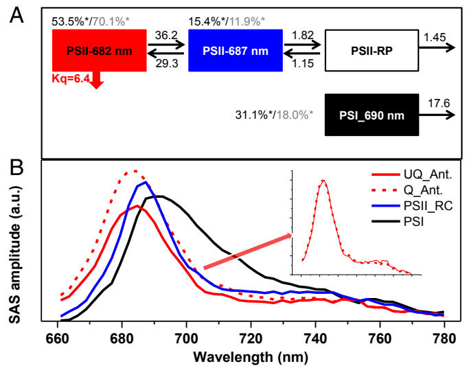
Fig. 3. Target analysis results. (A) Schematic model used to describe the time-resolved fluorescence data; rates are given in \text{ns}^{-1} , K_q is the rate of quenching, and asterisks indicate the initial excitations at 400 nm (black) and 475 nm (gray). (B) Species-associated spectra (SASs) of the compartments with the same colors as used in A. (B, Inset ) Normalized spectra of the UQ_Ant. and Q_Ant. are shown.
