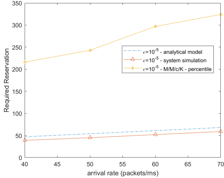
Fig. 8. System simulations versus analytical model.
