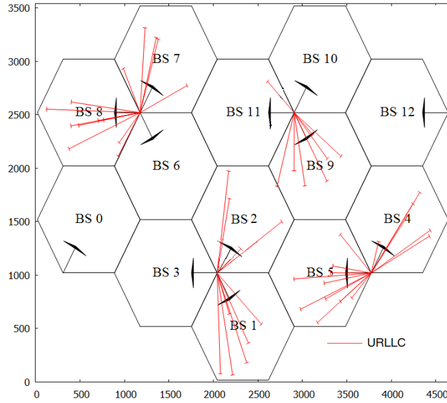
Fig. 7. Urban network with 13 gNodeBs.
