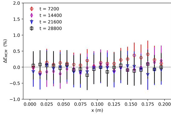
(c) Scaled differences with MCM confidence intervals for concrete (Case 1)
