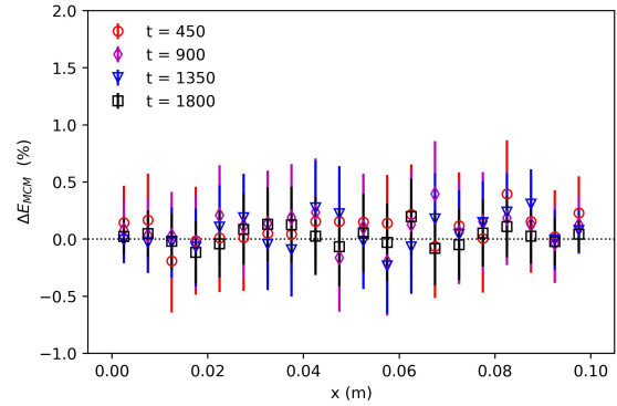
(d) Scaled differences with MCM confidence intervals for EPS (Case 1)
