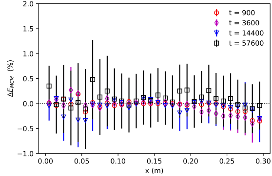
(f) Scaled differences with MCM confidence intervals for Case 2
