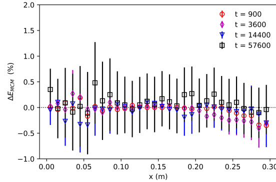
(f) Scaled differences with MCM confidence intervals for Case 2
