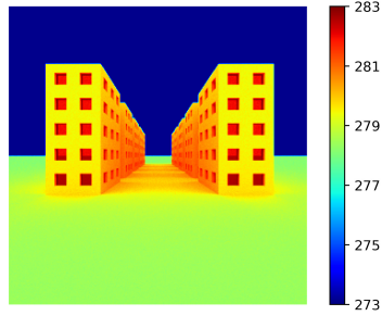
(d) Reference radiance temperature computed with HTRDR-Urban (Case 4)
