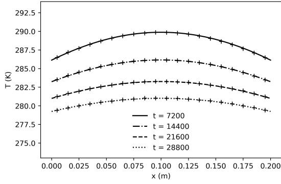
(a) Temperature profiles in concrete slab (Case 1)
