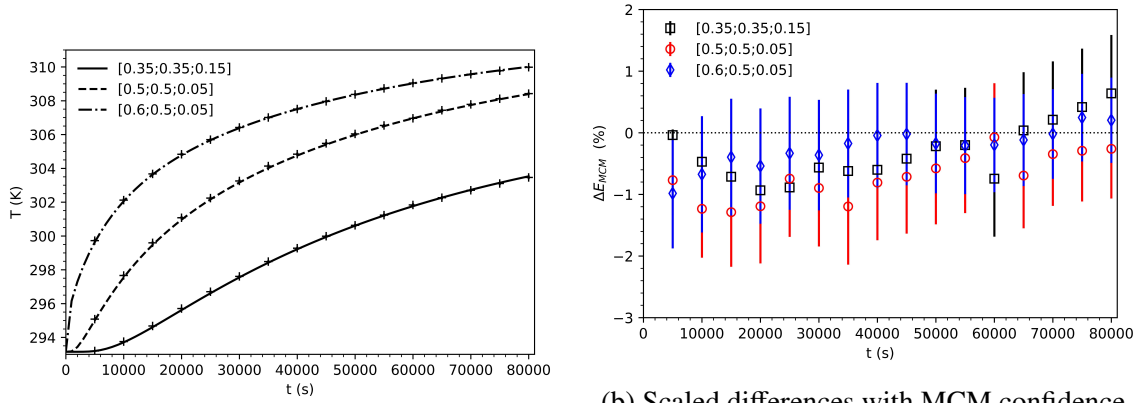
(a) Transient temperatures for three locations in Case 3
