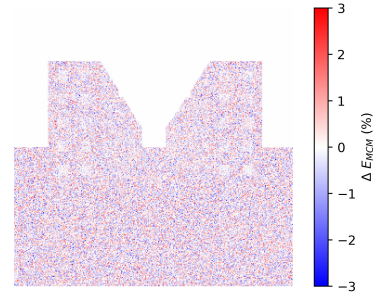
(e) Scaled differences between our code and HTRDR-Urban software (Case 4)
