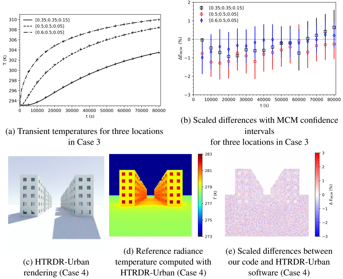
Figure 5: Numerical validation results of cases 3 and 4: Comparison of transient temperatures (a) for the thermal bridge Case 3 for three locations: Point [0.35; 0.35; 0.15] is located in the lower part of the insulation (EPS) corner; Point [0.5; 0.5; 0.05] is located inside the concrete part of the thermal bridge; Point [0.6; 0.5; 0.05] is located on the external (concrete) surface. Temperatures computed with OpenFoam are plotted with lines and the results of MCM are given with markers. The scaled numerical error (Eq. 24) with the MCM confidence intervals are given in (b); Rendering (c) in the visible spectrum ( 0.38\text{-}0.78\ \mu\text{m} , CIE XYZ [33]) with HTRDR-Urban [9, 8] of the complex geometry: two parallel rows of five aligned buildings; The walls are Lambertian and the windows are specular; Solar elevation is 45^\circ and azimuth is 120^\circ from north (clockwise). An infrared geometry rendering is shown in (d) with reference radiance temperatures computed with HTRDR-Urban. In (e) the pixel-based scaled differences between the present model and the reference are given (each image has a resolution of 300 \times 300 pixels)
