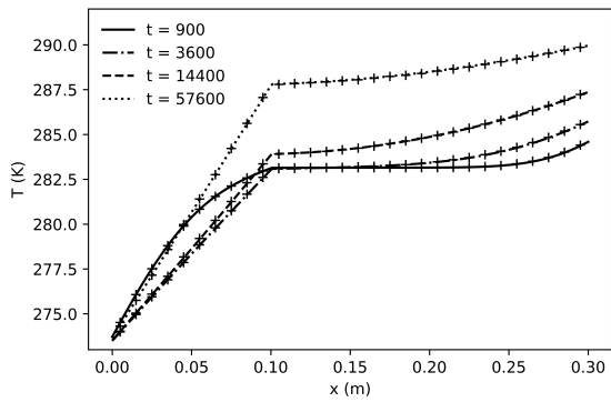
(e) Temperature profiles for Case 2
