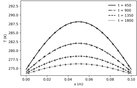
(b) Temperature profiles in EPS slab (Case 1)
