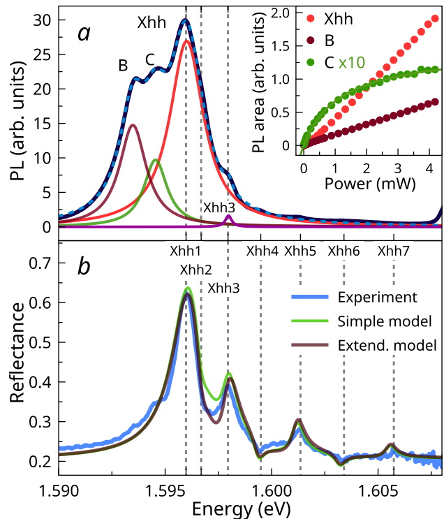
Figure 1. (a) PL spectrum measured at E_{\text{exc}} = 1.653 eV and P_{\text{exc}} = 0.6 mW. Laser spot diameter, d = 0.1 mm. Dashed curve is a fit to the data with the sum of four Lorentzians (solid lines). Inset shows the power dependence of integral areas of spectral the components labeled as Xhh, B, and C (points). Solid curves are linear approximations for the Xhh and B components and the approximation by function (2) with P_0 = 1.2 mW for the C component. (b) Reflectance spectrum (noisy curve) and its modeling in the framework of the simple and extended models (see the text for details). The calculated spectra are shifted by 2.15 meV and scaled using the factor 0.93. Vertical dashed lines marked X_{hh1} , X_{hh2} etc, indicate the energies of the quantum-confined heavy-hole exciton states. Sample temperature T = 4 K for both experiments.
