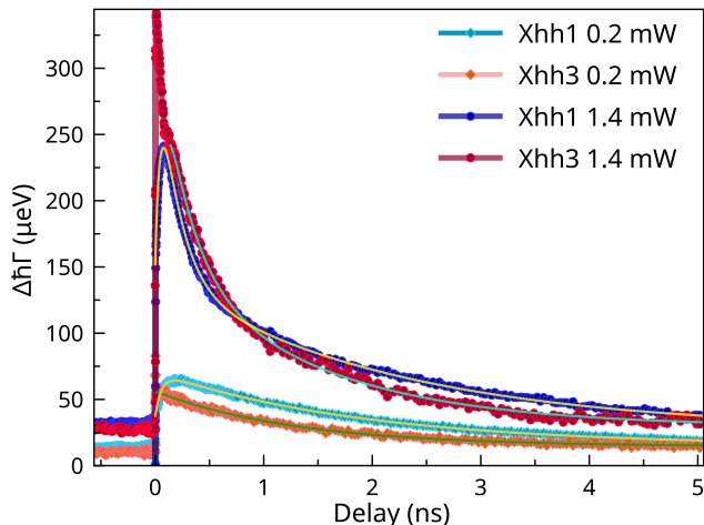
Figure 3. Dynamics of the photo-induced part of the nonradiative broadening of the resonances Xhh1 and Xhh3, powers are shown in the legend. Smooth solid curves are the fits by function (9) with the time constants given in Tab. III. Sample temperature T = 4 K.
