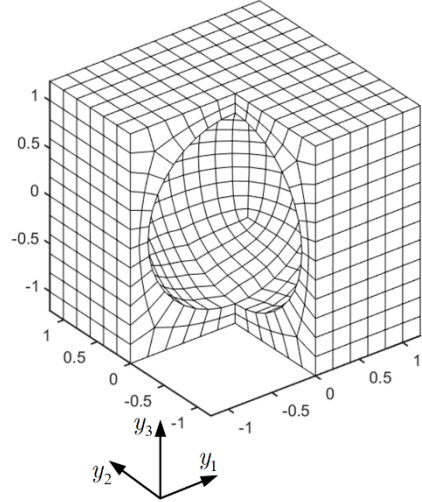
Figure 21 Finite element mesh refinement of the unit cell with spherical porosity
