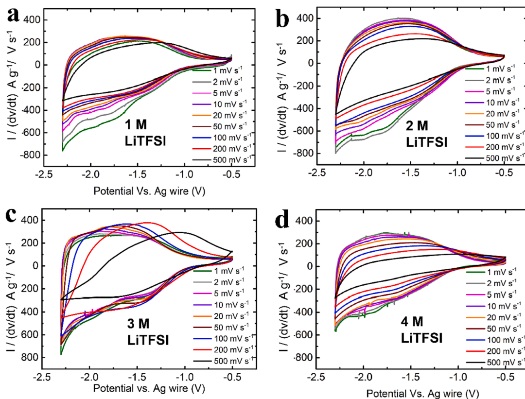
Fig. 3. CV curves of MS-Ti 3 C 2 T x recorded at various potential scan rates from 1 to 500 \text{ mV s}^{-1} within a potential window from -2.3 \text{ V} to -0.5 \text{ V} vs Ag for LiTFSI in ACN electrolytes at different concentrations: (a) 1 M, (b) 2 M, (c) 3 M and (d) 4 M.
