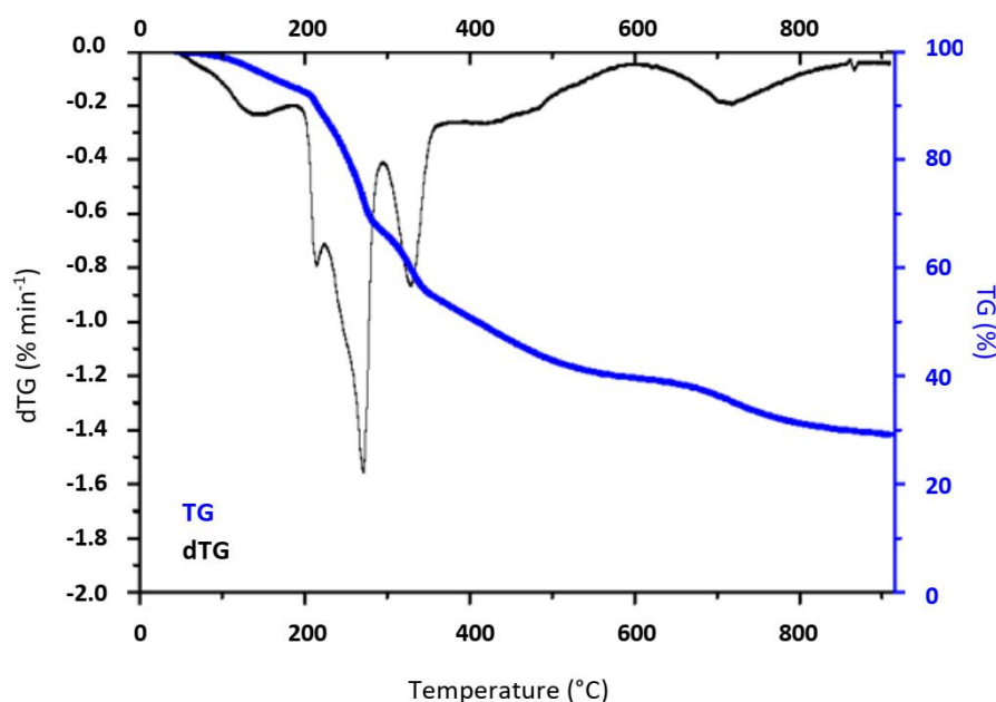
Figure 2. Thermogravimetric analysis profiles of as-received Sargassum algae ( S_{\text{raw}} ).
