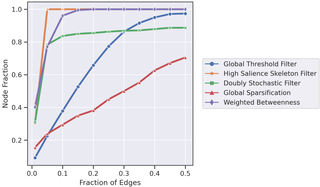
Figure 6. A line chart showing the fraction of nodes of the extracted structural backbones as a function of the fraction of edges plotted using netbone .
