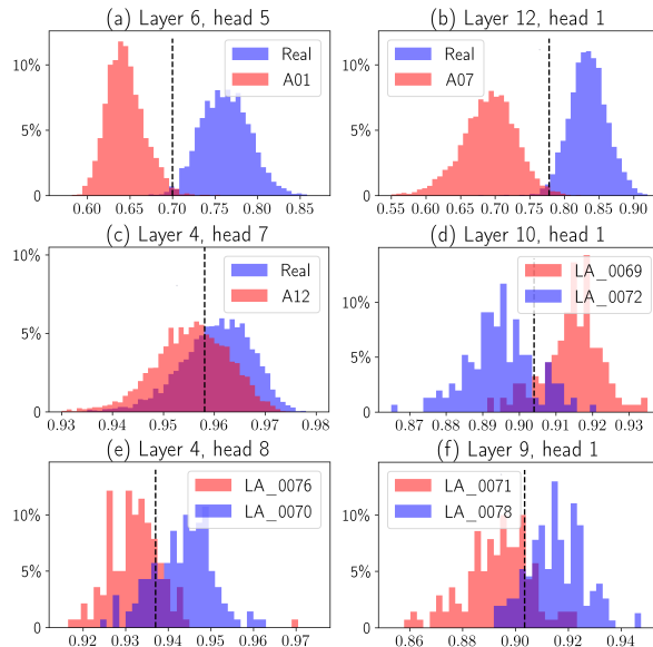
Figure 2: H_0^{m, \text{sym}} for the best HuBERT heads for two tasks: (a-c) individual model separation between human (blue) and synthetic (red) speech; (d-e) speaker separation; LA_0069, LA_0072, LA_0078 – female speakers, LA_0070, LA_0076, LA_0071 – male speakers.
