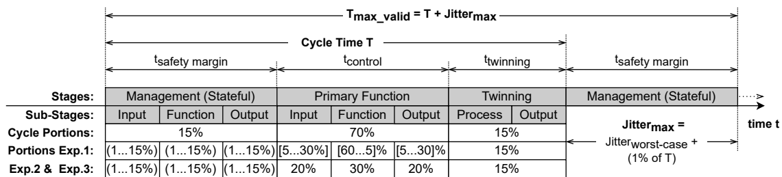
Figure 9. SA DT model specifying the timing constraints for the individual pipeline stages and sub-stages.
