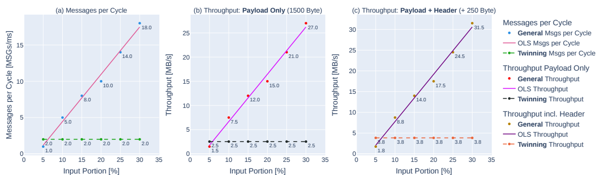
Figure 21. End-to-end throughput characteristics of the cyclic processing pipeline under different load conditions.
