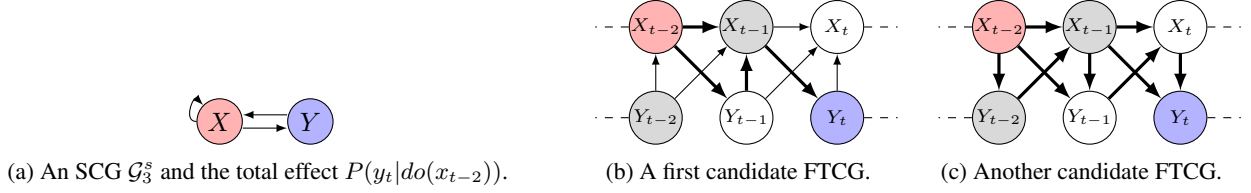
Figure 5.4: An example of an SCG \mathcal{G}_3^s in (a) satisfying Condition 2b in Theorem 2 with respect to \Pr(y_t | do(x_{t-2})) and two candidate FTCTGs in (b) and (c). Each pair of red and blue vertices in the FTCTGs represents the total effect we are interested in. Gray vertices are ambiguous: they constitute a backdoor path in (b) and belong to a directed path in (c) (bold edges indicate direct paths from X_{t-2} to Y_t ).
