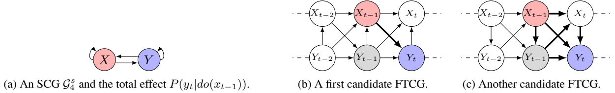
Figure 5.5: An example of an SCG \mathcal{G}_4^s in (a) satisfying Condition 2c in Theorem 2 with respect to \Pr(y_t | do(x_{t-1})) and two candidate FTCTGs in (b) and (c). Each pair of red and blue vertices in the FTCTGs represents the total effect we are interested in. Gray vertices are ambiguous: they constitute a backdoor path in (b) and belong to a directed path in (c) (bold edges indicate direct paths from X_{t-1} to Y_t ).
