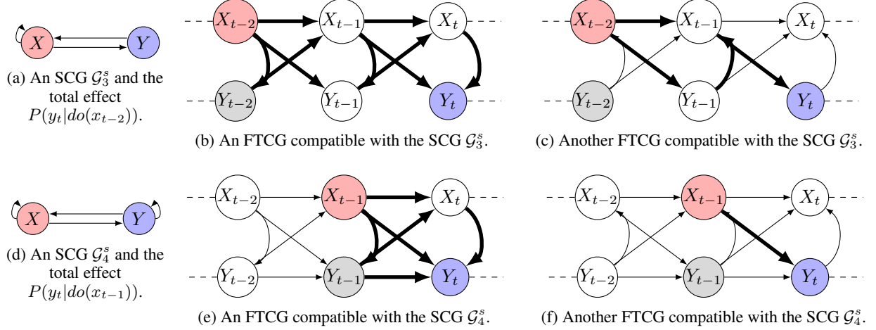
Figure 3: An example of an SCG \mathcal{G}_3^s in (a) (resp. \mathcal{G}_4^s in (d)) with two of its compatible FTCTs in (b) and (c) (resp. in (e) and (f)). Each pair of red and blue vertices in the FTCTs represents one total effect we are interested in. Gray vertices are ambiguous, and bold edges correspond to direct path from X_{t-\gamma} to Y_t . In both examples, the total effect is not identifiable given the SCG as stated in Lemma 3 (resp. Lemma 4).
