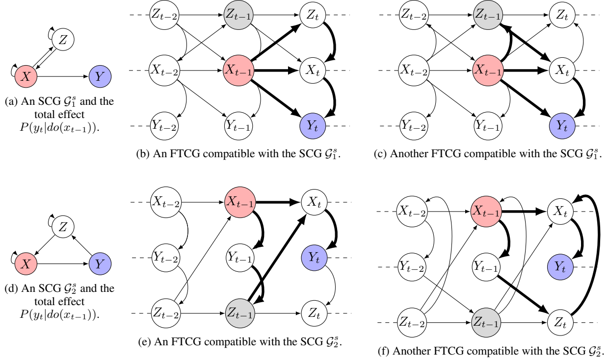
Figure 2: An example of an SCG \mathcal{G}_1^s in (a) (resp. \mathcal{G}_2^s in (d)) with two of its compatible FTCCGs in (b) and (c) (resp. in (e) and (f)). Each pair of red and blue vertices in the FTCCGs represents one total effect we are interested in. Gray vertices are ambiguous, and bold edges correspond to direct path from X_{t-\gamma} to Y_t . In both examples, the total effect is not identifiable given the SCG as stated in Lemma 1 (resp. Lemma 2).
