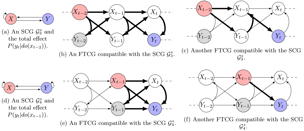
Figure 3: An example of an SCG \mathcal{G}_3^s in (a) (resp. \mathcal{G}_4^s in (d)) with two of its compatible FT CGs in (b) and (c) (resp. in (e) and (f)). Each pair of red and blue vertices in the FT CGs represents one total effect we are interested in. Gray vertices are ambiguous, and bold edges correspond to direct path from X_{t-\gamma} to Y_t . In both examples, the total effect is not identifiable given the SCG as stated in Lemma 3 (resp. Lemma 4).
