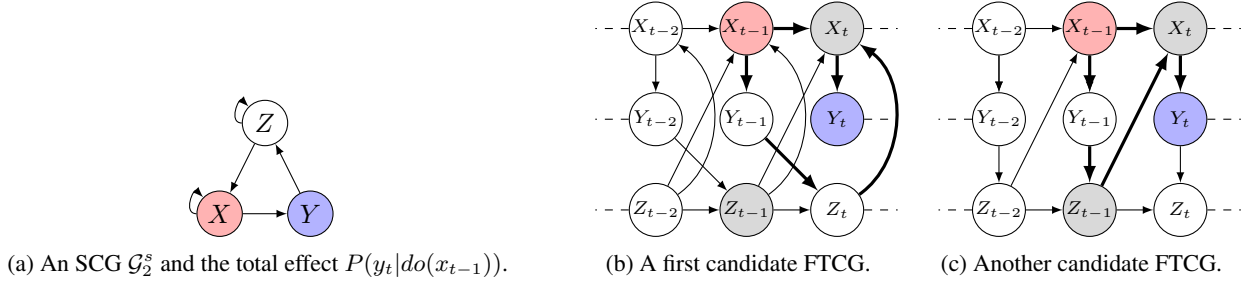
Figure 5.3: An example of an SCG \mathcal{G}_2^s in (a) satisfying Condition 2a in Theorem 2 and two candidate FTFCGs in (b) and (c). Each pair of red and blue vertices in the FTFCGs represents the total effect we are interested in. Gray vertices are ambiguous: they are on an active backdoor path in (b) and belong to a directed path in (c) (bold edges indicate direct paths from X_{t-1} to Y_t ).
