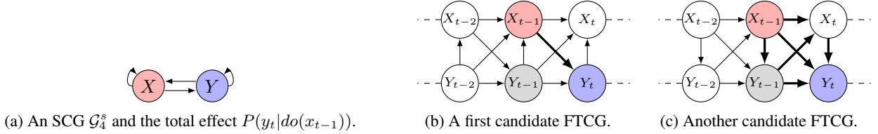
Figure 5.5: An example of an SCG \mathcal{G}_4^s in (a) satisfying Condition 2c in Theorem 2 with respect to \Pr(y_t | do(x_{t-1})) and two candidate FTFCGs in (b) and (c). Each pair of red and blue vertices in the FTFCGs represents the total effect we are interested in. Gray vertices are ambiguous: they constitute a backdoor path in (b) and belong to a directed path in (c) (bold edges indicate direct paths from X_{t-1} to Y_t ).
