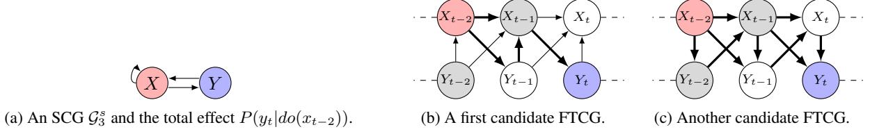
Figure 5.4: An example of an SCG \mathcal{G}_3^s in (a) satisfying Condition 2b in Theorem 2 with respect to \Pr(y_t | do(x_{t-2})) and two candidate FTFCGs in (b) and (c). Each pair of red and blue vertices in the FTFCGs represents the total effect we are interested in. Gray vertices are ambiguous: they constitute a backdoor path in (b) and belong to a directed path in (c) (bold edges indicate direct paths from X_{t-2} to Y_t ).
