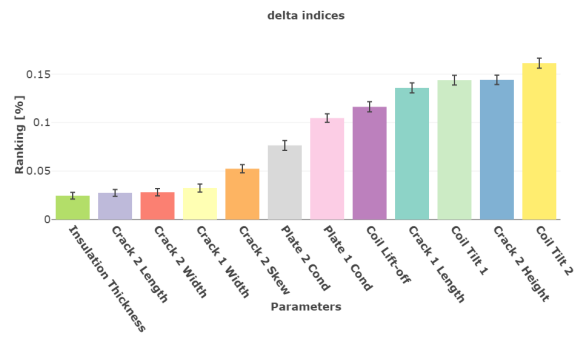
Figure 7: Results of global sensitivity analysis through \delta -importance index. In (a), the results obtained from the extraction based on the L_2 -norm calculation performed on the absolute value of C-scan ECT signals. In (b) and (c) the results display the same calculation performed in (a), based on real and imaginary part of \Delta Z , respectively.
