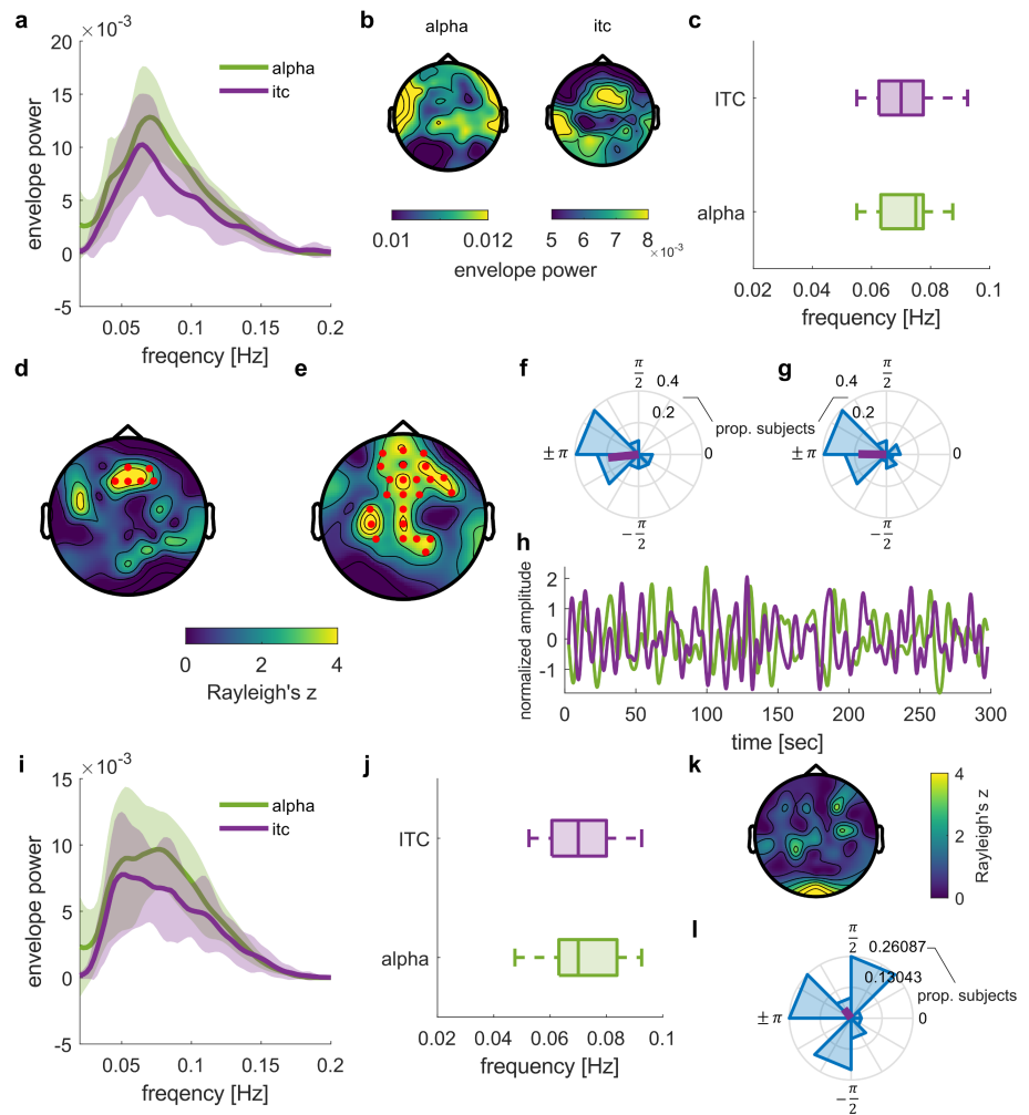
Figure 2: \alpha -power and entrainment exhibit slow anti-phase fluctuations. (a-h) Results for eyes-open condition. (a) Envelope spectra of \alpha -power and entrainment to rhythmic speech show a peak around 0.07-Hz (shown for electrode Fz). Shaded areas depict standard deviation. (b) Topography of the 0.07-Hz peak shown in a. (c) Distribution of individual peak frequencies from the spectra shown in a. (d) Coupling between \alpha -power and entrainment fluctuations around 0.07-Hz when both were extracted from the same channel. Channels showing a significantly non-uniform distribution of phase differences are highlighted in red, topography indicates the underlying z-statistic. (e) Channels showing significant coupling between \alpha -power fluctuations per channel with entrainment in the frontal cluster (d). (f) Distributions of phases in channels showing significant \alpha -power vs. entrainment coupling (cluster shown in d). \alpha -power and entrainment to speech are coupled in anti-phase. (g) \alpha -power fluctuations in cluster shown in (e) are coupled in anti-phase. (h) Exemplary time-course of \alpha -power and entrainment fluctuations at electrode Fz. (i-l) same as a, c, d, g, but for eyes-open condition.
