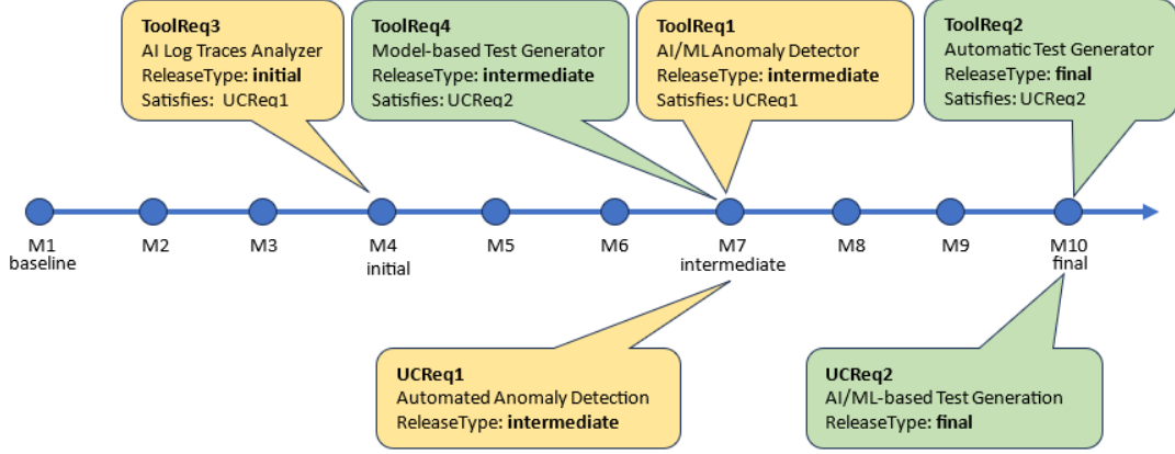
Figure 11: Generic example of creating the roadmap for use case requirements validation.
