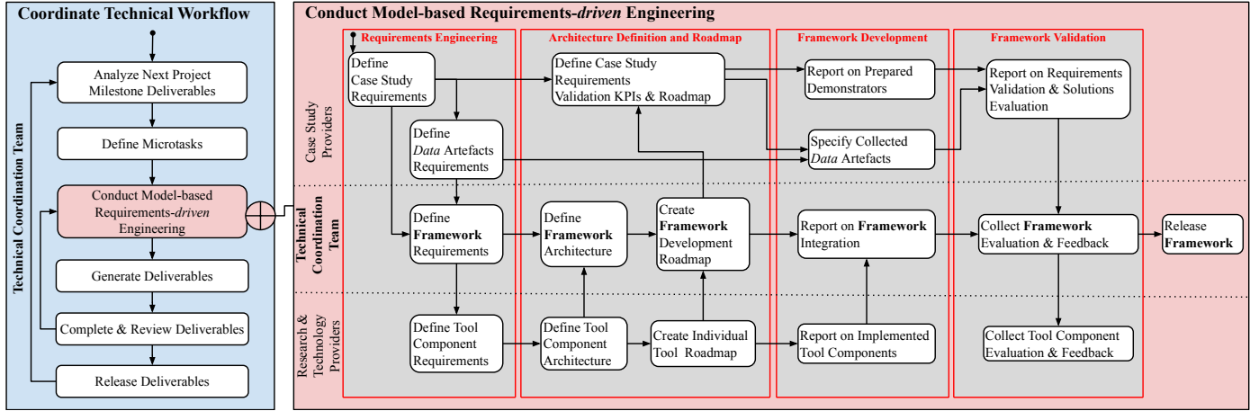
Figure 1: Our Iterative Model-based Requirements Engineering Conceptual Approach.
