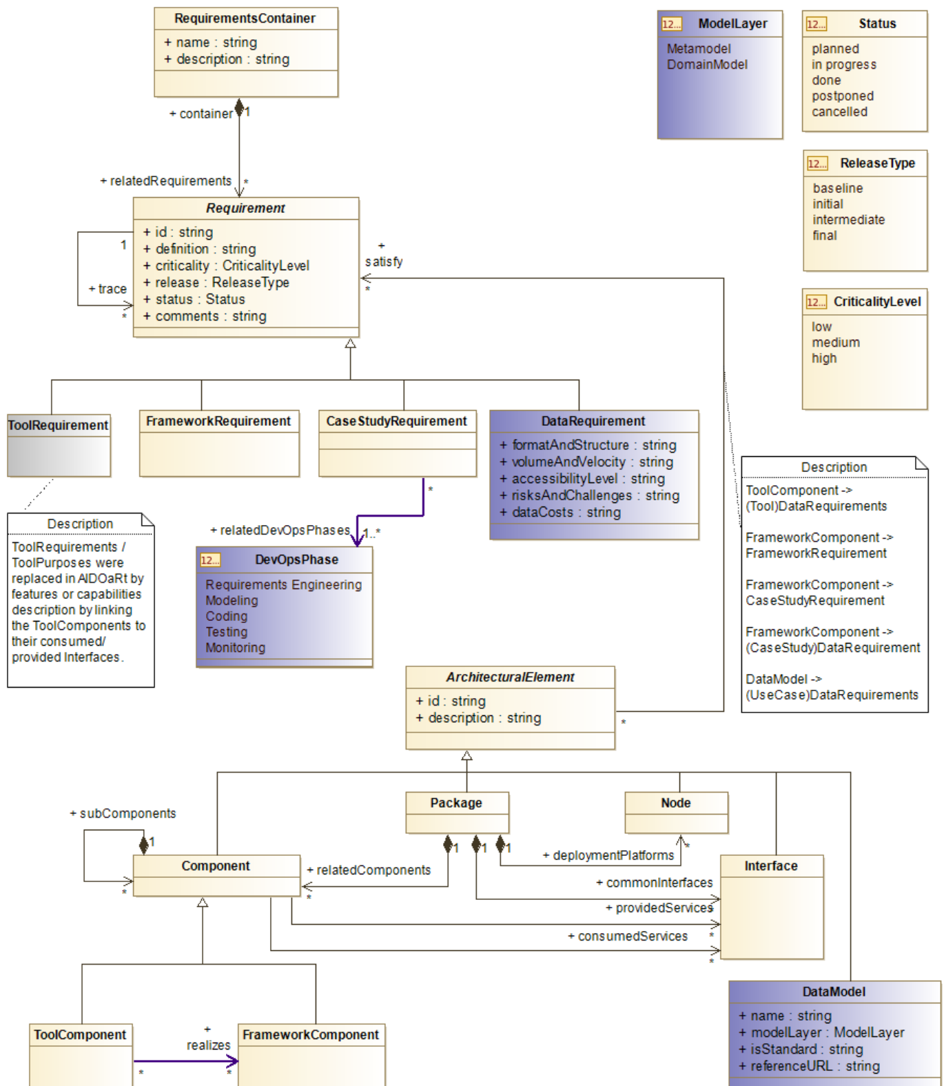
Figure 3: Metamodel of our Extended RE Language (elements in purple depict the newly added concepts to the abstract syntax of our language).
