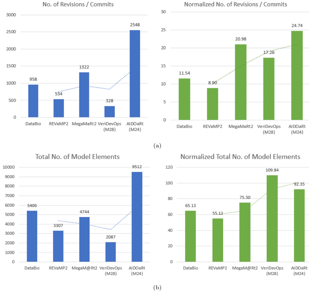
Figure 12: Figure (a) shows the evolution of the total number of commits or revisions made by the project members to their model repositories, and Figure (b) shows the total number of created model elements. The left charts show the raw numbers, whereas the right charts show these numbers normalized w.r.t. to the size of the projects (i.e., the number of partners, case studies, and solutions). The dotted curves illustrate the moving average trends.
