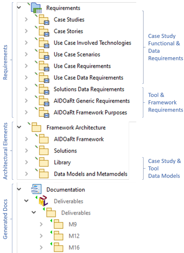
Figure 5: Structure of the enriched RE model in Modelio: Example from the AIDOaRt project.
