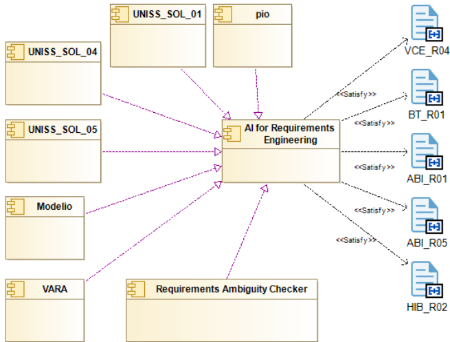
Figure 9: Traceability diagram in Modelio: Example from AIDOaRt showing the mapping between an architecture component, related solutions, and case study requirements.
