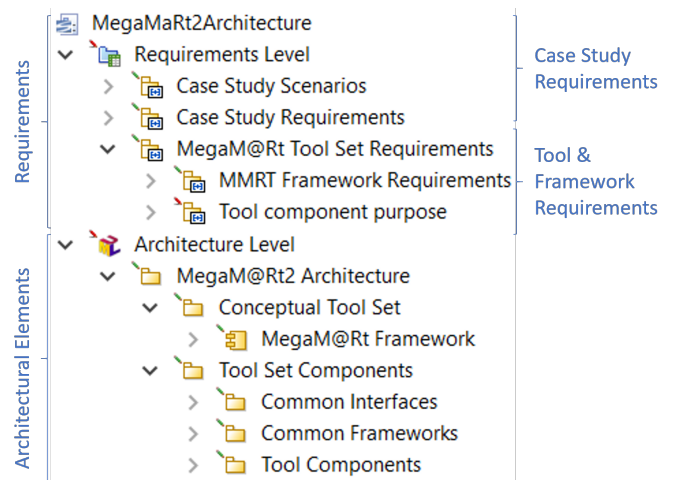
Figure 4: Structure of the base RE model in Modelio: Example from the MegaM@Rt2 project.
