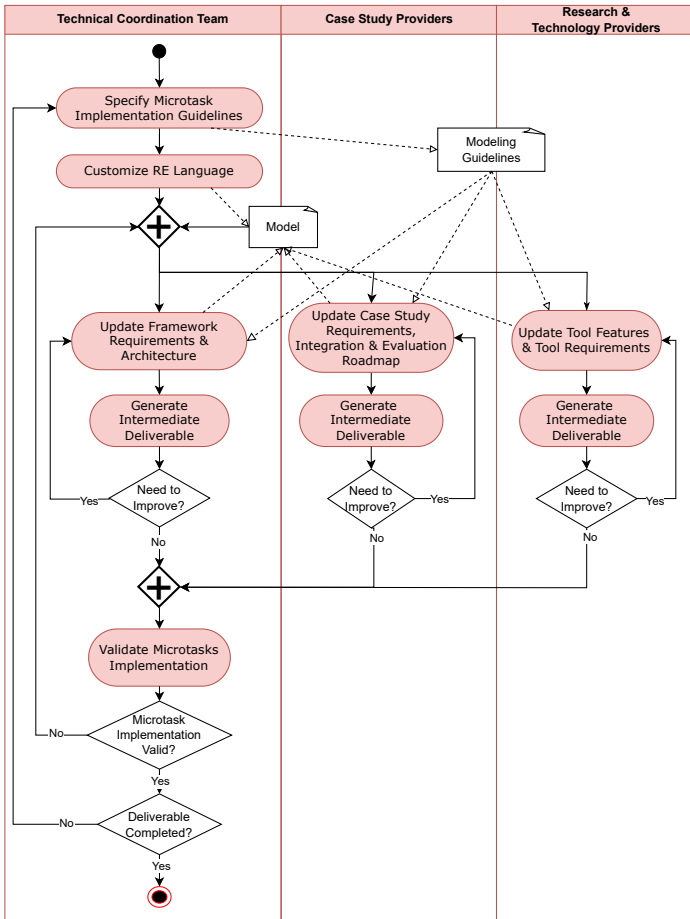
Figure 2: Iterative process of our MBRE Approach: iterative model extensions and continuous updates timely support the project's evolution and the deliverables creation process.
