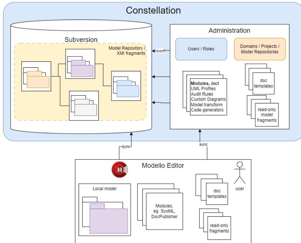
Figure 6: High-level view of the Modelio and Constellation solutions for collaborative modeling support.
