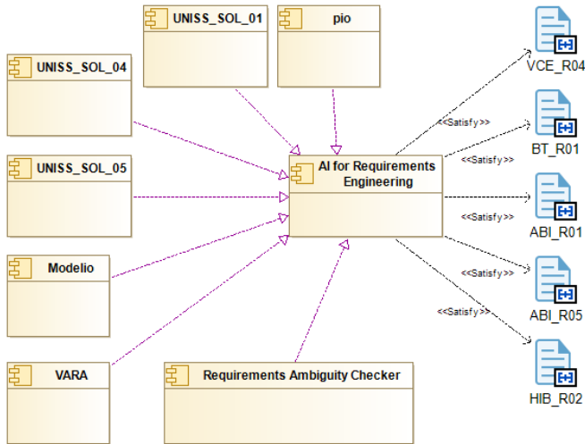
Figure 9: Traceability diagram in Modelio: Example from AIDOaRt showing the mapping between an architecture component, related solutions, and case study requirements.
