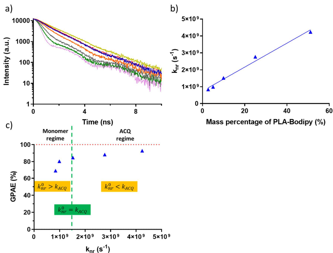
Figure 4. (a) Fluorescence decays of NP solution, excitation at 781 nm with a pulsed diode <200 ps, emission at 820 nm. (Yellow, Bodipy NP-2.5%), (Red, Bodipy in DCM), (blue, Bodipy NP-5%), (orange, Bodipy NP-10%), (grey, Bodipy NP-25%), (green, Bodipy NP-50%), (purple, excitation diode signal). (b) Evolution of the non-radiative rate constant k_{nr} as a function of the introduced mass percentage of PLA-Bodipy. The rate constants were determined thanks to the Strickler-Berg equation. Absorbance linear fit: R^2 = 0.9869 and y = 7.08 \times 10^7 x + 7.44 \times 10^8 . (c) Evolution of the GPAE as a function of the non-radiative rate constant. The red line represents the curve GPAE = 100%.
