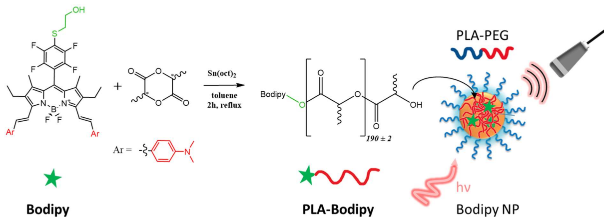
Figure 1. Molecular structure of the Bodipy and PLA-Bodipy and schematic representation of the photoacoustic activated Bodipy NP.
