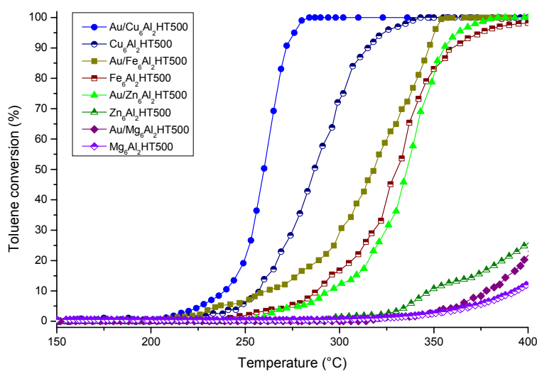
Figure 3. Toluene conversion on mixed oxide supports and gold catalysts vs. reaction temperature.
