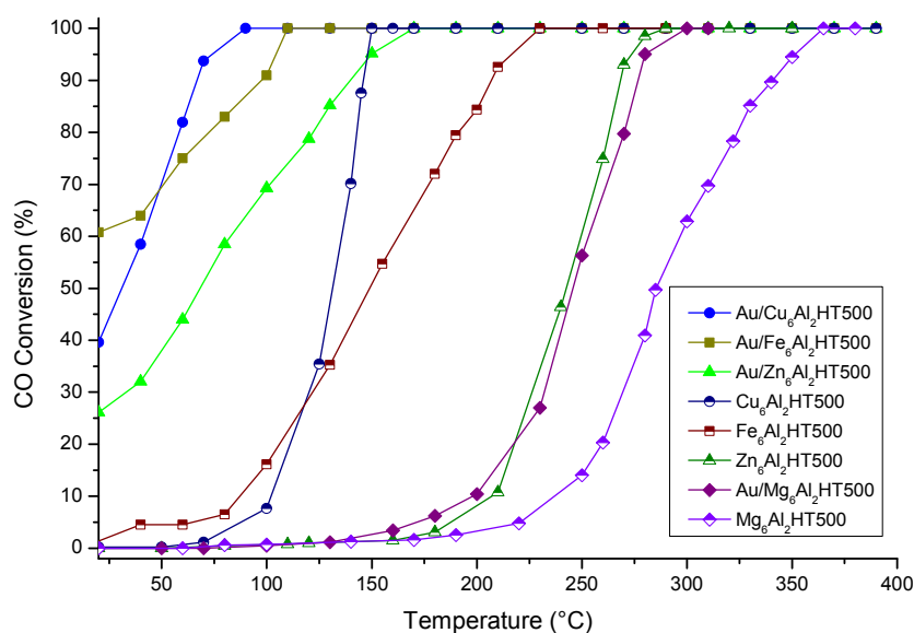
Figure 4. Carbon monoxide conversion on mixed oxide supports and gold catalysts vs. reaction temperature.
