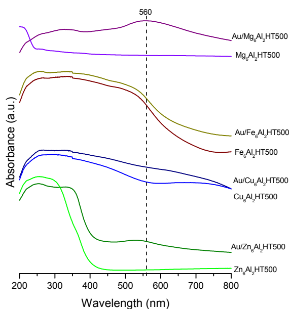
Figure 2. UV–visible diffuse reflectance (DR-UV-vis) spectra of X 6 Al 2 HT500 support and Au/X 6 Al 2 HT500 gold based catalysts.
