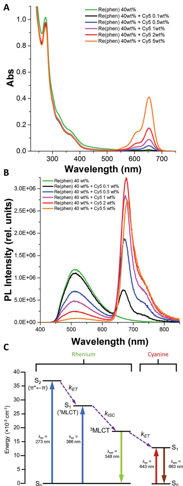
Figure 4. A) Absorption spectra of NPs loaded with 40 wt.% of Re(phen) and increasing amounts of Cy5. B) PL spectra of the same NPs excited at \lambda_{ex} = 292\text{ nm} C) Simplified energy level diagram for downshifting energy transfer processes within Re(phen) and Cy5-loaded NPs.
