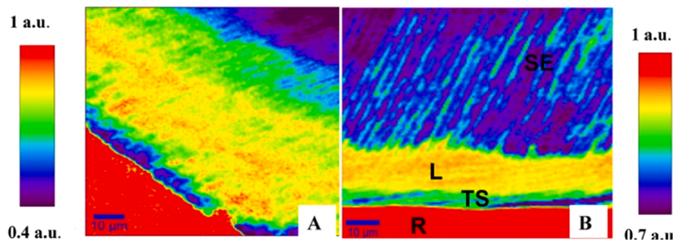
Fig. 6. FTIR mapping of (A) natural lesions and (B) chemically-induced caries. Images are constructed from the ratio between the intensity of the carbonate and phosphate vibration bands. Reproduced from [52] – Creative Commons CCBY.
