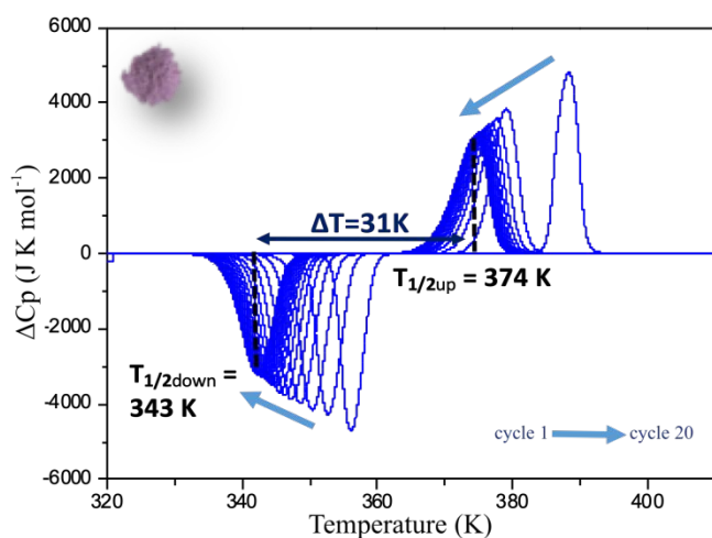
Figure 3. Deviation from normal molar heat capacity ( \Delta C_p ) vs temperature for 1 recorded by DSC on a powder sample at 5 K \text{min}^{-1} . Arrows are showing the evolution from the first to the 20 th cycle. \Delta C_p peaks in the cooling mode are artificially represented negatives, that way, endothermic process correspond to a positive peak in the chart.
