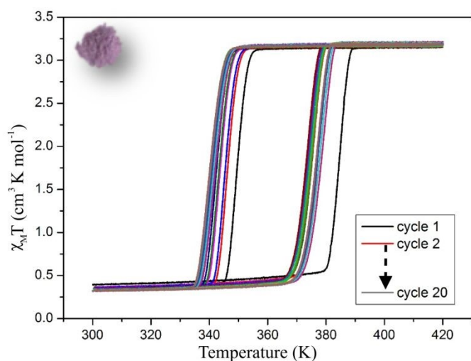
Figure 2. \chi_M T product versus T recorded on a powder sample of 1 showing the evolution of the magnetic properties upon 20 cycles. Scan rate = 5 K \text{min}^{-1}
