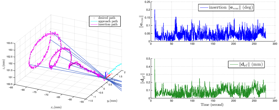
(a) the path performed by a straight tool under the RCM constraints (b) the alignment error \mathbf{e}_{rcm} and that of the path following \mathbf{d}_{pf}
