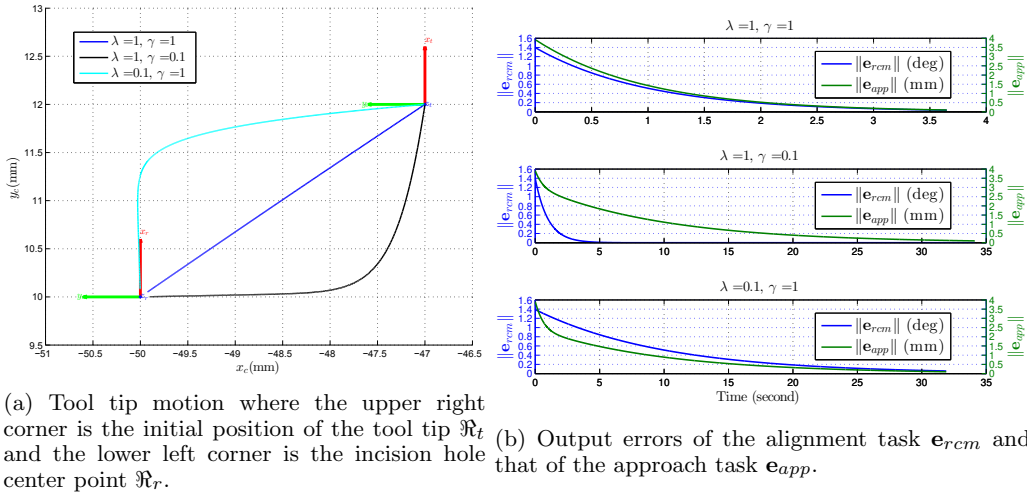
Fig. 12: The system performances during the outside phase while varying the values of \lambda and \gamma .
