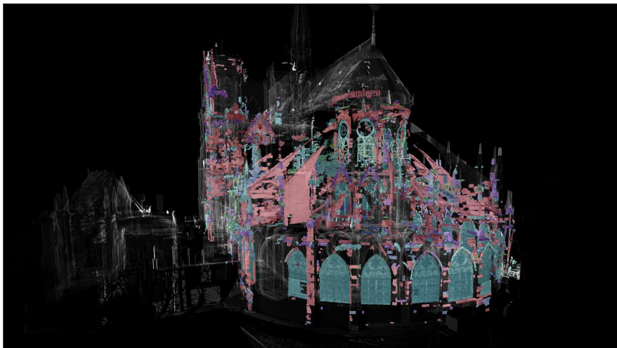
Figure 15: Import of the 113 Aioli projects of the architectural diagnosis of Notre-Dame in a third-party viewer, superimposed with other 3D resources including a 3D point cloud of the cathedral (before fire) from a lasergrammetric survey conducted by Andrew Tallon (Vassar College) between 2006 and 2012.
