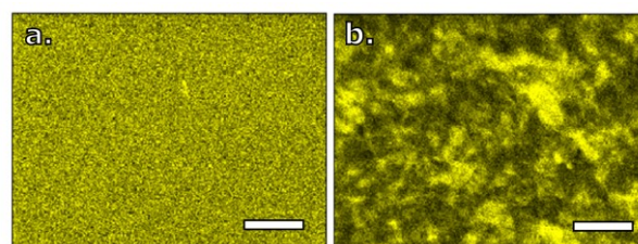
Fig. 1 Distribution of sulfur by EDX in PEDOT:PSS/PEO processed by DC (a) and ExTC (b) (Scale bar: 25 \mu m).
