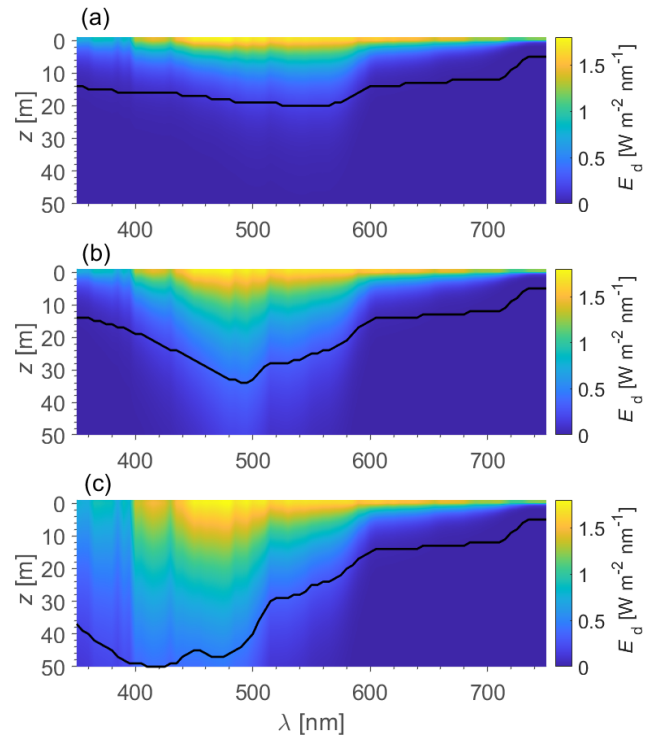
Figure 12. Examples of depth profiles of E_d(z, \lambda) for a given IOP scenario from (a) OWG 1, (b) OWG 2, and (c) OWG 3. Radiative transfer simulations were performed for a sun zenith angle of 30^\circ and included Raman scattering by water molecules and chlorophyll a fluorescence. The black line depicts the first optical attenuation depth, z_1
