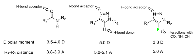
Scheme 5. 5-F triazole in comparison to amide bond and 5-H triazole
