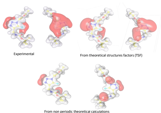
Fig. 4. Experimental and theoretical electrostatic potential for two orientations of molecule 2a . Isovalue surface cut-off is +0.1 \text{ e/bohr} (in grey) and -0.05 \text{ e/bohr} (in red).
