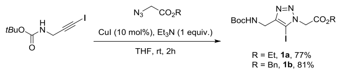
Scheme 1. Synthesis of 5-iodo-1,2,3-triazoles
