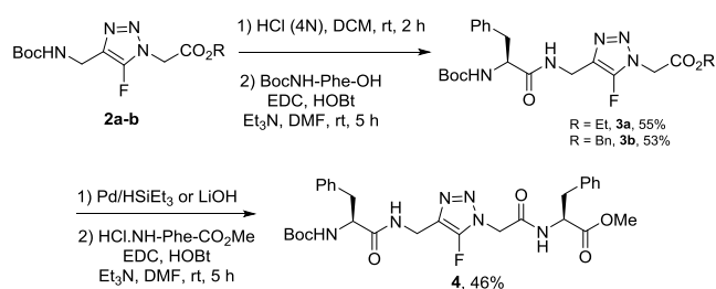
Scheme 3. Incorporation of amino acids
