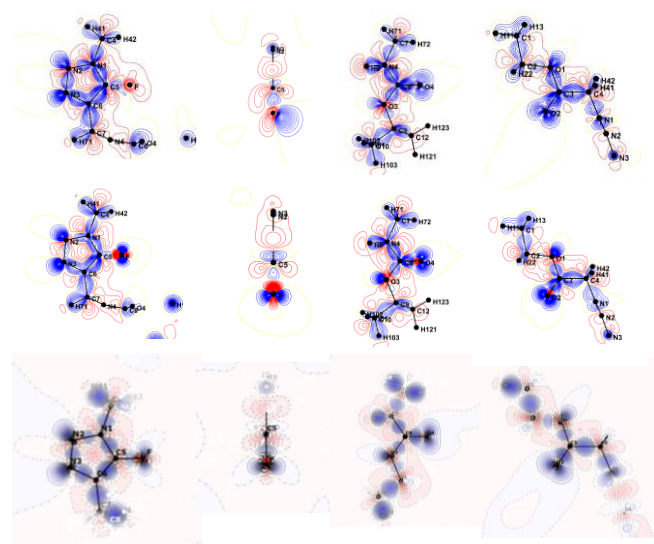
Fig. 3. Experimental static electron deformation density (top) and theoretical ones (from TSF refinement, middle and isolated molecule, bottom) in chosen planes of molecule 2a . Contours are 0.05 \text{ e}\text{\AA}^{-3} , negative contours are in red.
