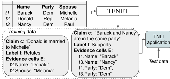
Fig. 1. Given any table, TENET generates new training examples for a target TNL application. The first example has a hypothesis that is refuted according to the data evidence.
