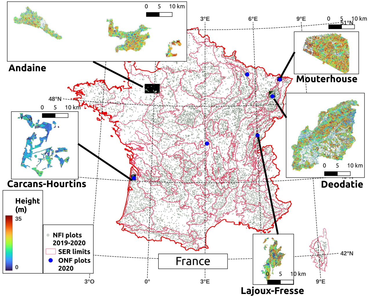
Figure 3. Validation data: ALS-CHM from ONF on 5 test sites, NFI plots (grey points), ONF plots (blue points) and SER (boundaries in red).
