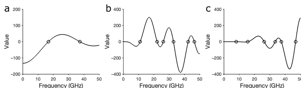
Figure A1. Evaluation of eigenvalue equations for a sphere with R = 50 nm, V_l = 1920 m/s, and V_t = 960 m/s. Circles denote the roots. (a) Breathing mode ( l = 0 , Equation (A2)). (b) Dipolar mode ( l = 1 , Equation (A1) or (A4)). (c) Quadrupolar mode ( l = 2 , Equation (A1) or (A5)).
