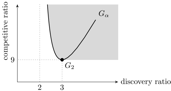
Fig. 2 Every strategy X corresponds to a point with coordinates \text{dr}(X) and \text{cr}(X) , which belongs to the region depicted in gray. Its Pareto boundary is constituted by the geometric strategies G_\alpha for \alpha > 1 .
