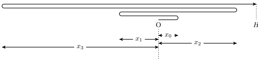
Fig. 1 An illustration of a search strategy determined by the sequence \{x_0, x_1, \dots\} .
