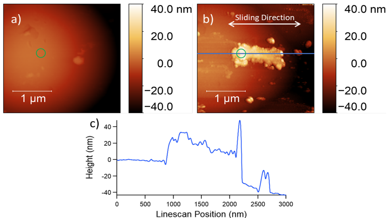
Figure 3: (a) Topographic contact-mode AFM image of steel colloid prior to reciprocating sliding test. (b) Topographic tapping-mode image of colloid after the reciprocating sliding test at 2.9 \mu\text{N} applied load shown in Figures 1 and 2. Green circles represent nominal contact area determined from DMT contact mechanics for bare a-C:H:Si:O/steel. (c) Linescan from (b).
