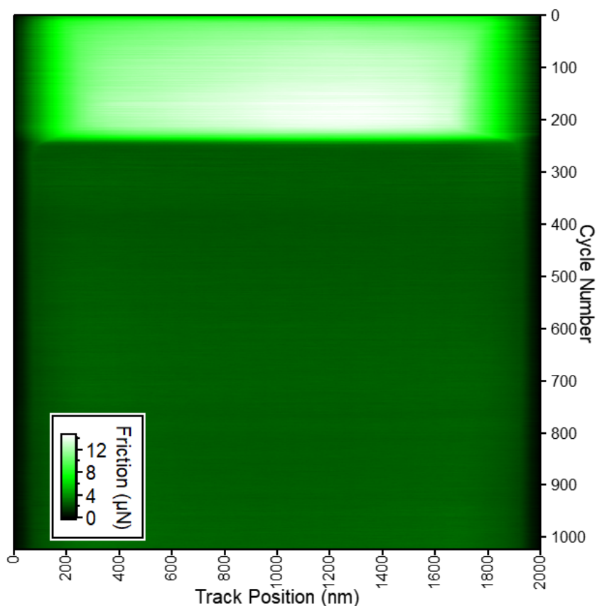
Figure 2: Friction force as a function of sliding cycles during reciprocating sliding of the steel colloid on a-C:H:Si:O in 50%RH N 2 with a 2.9 \mu N load. Horizontal features correspond to changes in time, vertical features, if present, would indicate changes to particular wear track regions.
