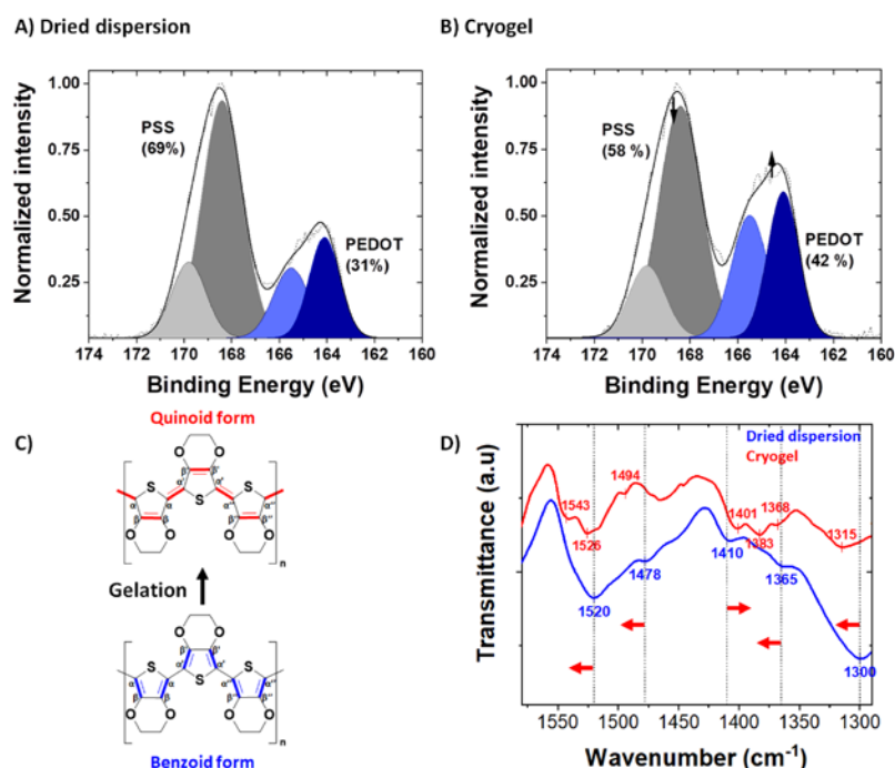
Figure 3 : A) S 2p XPS spectrum of the dried PEDOT:PSS dispersion (self-supported drop casted film); B) S 2p XPS spectrum of the quenched cryogel. (The molar % ratio is obtained via peak integration in grey for the PSS and blue for the PEDOT; gelation reduced the PSS
