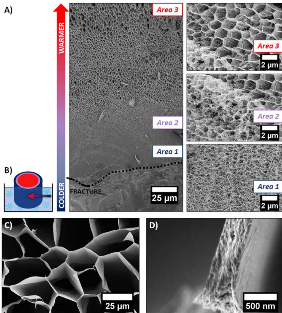
Figure 4 : A) cryo-SEM images of a unidirectional frozen piece of PEDOT:PSS hydrogel. Area 1 was in direct contact with liquid ethane, thus the native gel structure was preserved. Areas 2 and 3 show the evolution of the structure as the freezing rate decreased in the core of the sample; B) Schematic of the gel piece immersed in liquid ethane; the outer part in blue was in direct contact with the freezing solvent, resulting in the formation of amorphous ice. Deeper in the sample the freezing rate decreased, resulting in the formation of ice crystals. C) High magnification SEM image of the quenched cryogel showing the porous honeycomb-like structure. The channels are perfectly oriented towards the SEM detector in this area, D) SEM image of the pore wall structure of a quenched cryogel.
