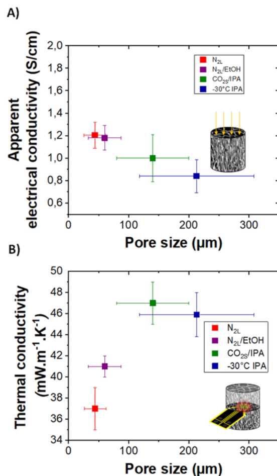
Figure 7 : A) and B) Apparent electrical conductivity and thermal conductivity of templated cryogels with different pore sizes, respectively.
