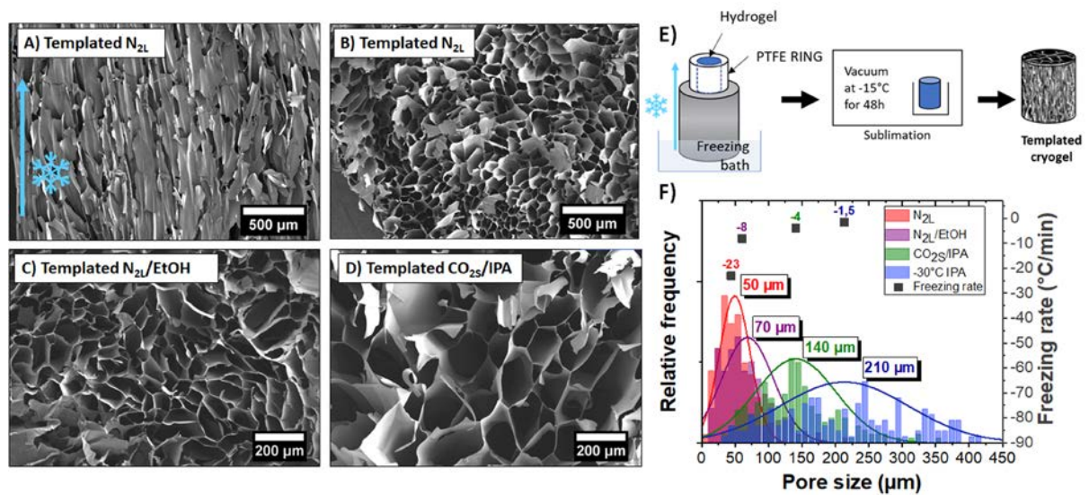
Figure 5 : A) Vertical and B) horizontal cut of a templated cryogel in N_{2L} ; C) and D) Horizontal SEM images at the same scale as of a templated cryogel in N_{2L} /EtOH and of a templated cryogel in CO_{2S} /IPA baths, respectively. The “flakes” lying on top of the pore surfaces are due to the cutting of the sample and are not representative of the real structure. E) Schematic of the ice-templating method used here to produce porous controlled PEDOT:PSS cryogels; F) Histogram of pore sizes measured in the quenched N_{2L} cryogel and in four templated cryogels produced at different freezing temperatures, the diameters are measured from SEM images. The second y- axis represents the freezing rate, measured with a thermocouple on top of the gel during freezing.
