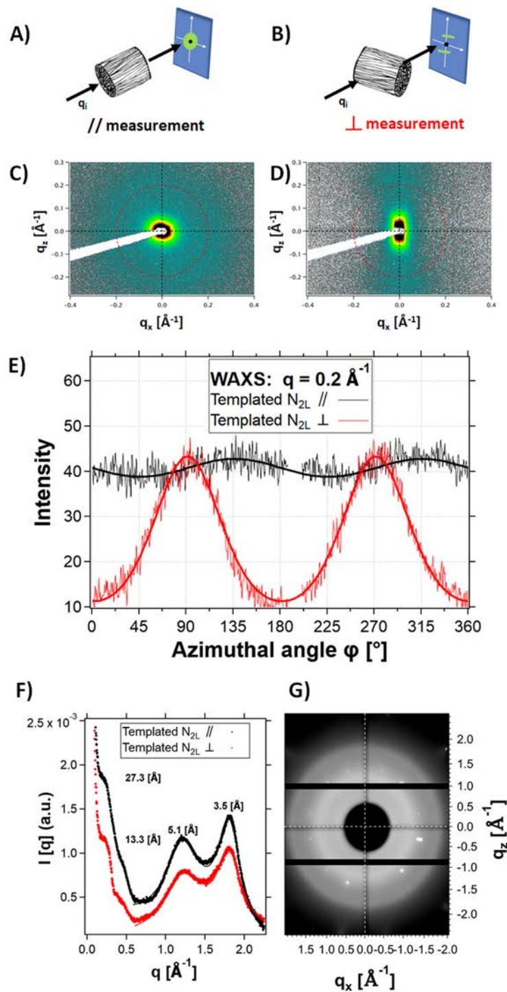
Figure 6: Schematics of the SAXS-WAXS measurements with the channels oriented parallel to the incident beam (A) or perpendicular to it (B). C and D) 2D detector images of the WAXS profile of a templated N_{2L} cryogel in the A) // , and B) \perp directions; E) azimuthal intensity profile of the templated N_{2L} cryogel measured in the // (black) and \perp (red) directions; F) SAXS and WAXS intensity profiles; G) 2 D detector images of the WAXS profile at wider angles ( > 1
