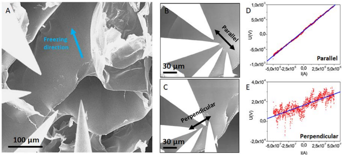
Figure 8: Mesoscopic measurements of electrical transport on the pore wall of a templated N_{2L} cryogel. A) SEM image of the four probes and the measured self-standing tube. The blue arrow indicates the direction of freezing. B and C) SEM images of the four-probes in a collinear arrangement, aligned along or perpendicular to the channel (to the freezing direction), respectively. D and E) Typical V(I) curves for the two orientations, parallel and perpendicular, respectively. The noise on the V(I) curve and the choice of the range of the applied current depended on the stability of the probes during the measurements (sometimes the tube deformed during the measurement). The measurements in the parallel
