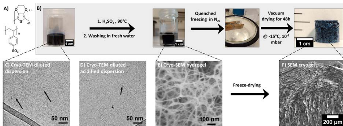
Figure 1: A) Chemical structure of PEDOT:PSS, B) process to form PEDOT:PSS hydrogel and quenched cryogel from the dispersion state, C-F) Inner structures observed by electron microscopy: C) cryo-TEM image of the diluted PEDOT:PSS dispersion. The black arrows highlight fibrils, D) cryo-TEM image of the acidified dispersion composed of long fibrils (black arrow). The fibrils are slightly more contrasted and more numerous than in the dispersion state (at a similar dilution). The black arrow head show a fibril pointing out of the image, along the electron beam, E) cryo-SEM image of the hydrogel, F) SEM image of the macroporous quenched cryogel. The porous channels appear locally oriented (on 300- 500 \mu\text{m} scale) but different orientations co-exist at the sample scale (1 cm) oriented in many different directions.
