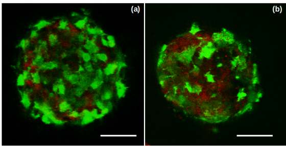
Fig. 3: Confocal microscopy images of spheroids prepared using T24 cells, at different initial collagen contents (a) c_0 = 0.01 mg/mL, (b) c_0 = 0.03 mg/mL. Scale bar 100 \mu\text{m} .
