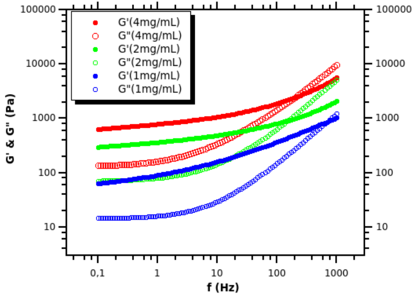
Figure 4: Predictions of the two-phase emulsion model for 80% cell volume concentration, \alpha/R=10^3 Pa, at collagen contents c = 1 mg/mL, 2 mg/mL and 4 mg/mL.
