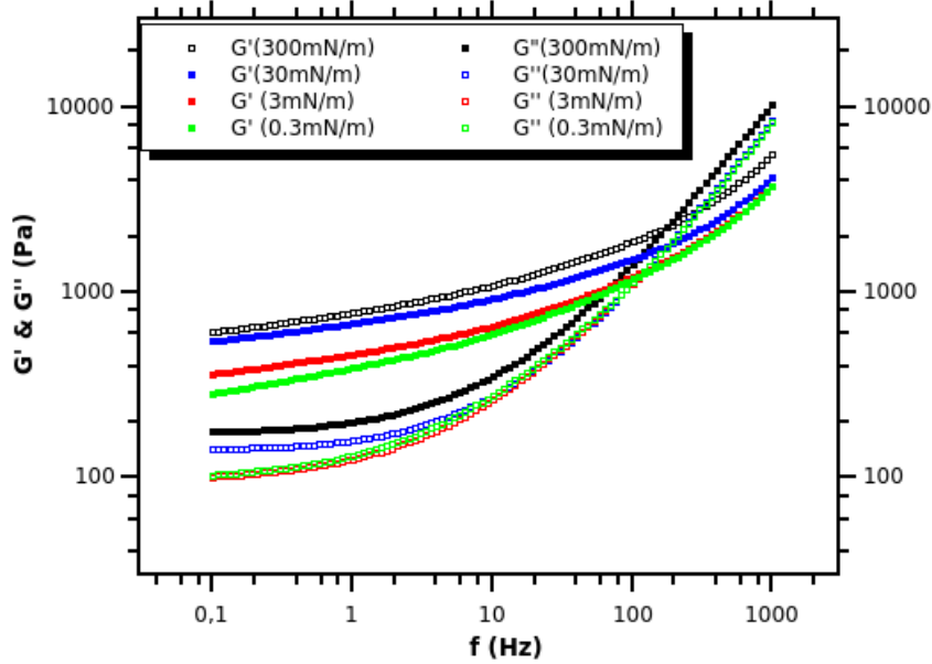
Figure 6: Predictions of the two-phase emulsion model for various adhesion energies \alpha=0.3 -3-30-300 mN/m, with R=10 \mu\text{m} , collagen content c = 2 \text{ mg/mL} , and \phi=0.9 .
