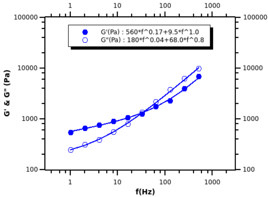
Figure 2: Rheological data of a T24 cell, measured at the surface of the spheroid, as a close representation of the cell's environment. Average of N=20 measurements, using 10 spheroids at c_0=0.01\text{mg/mL} .
