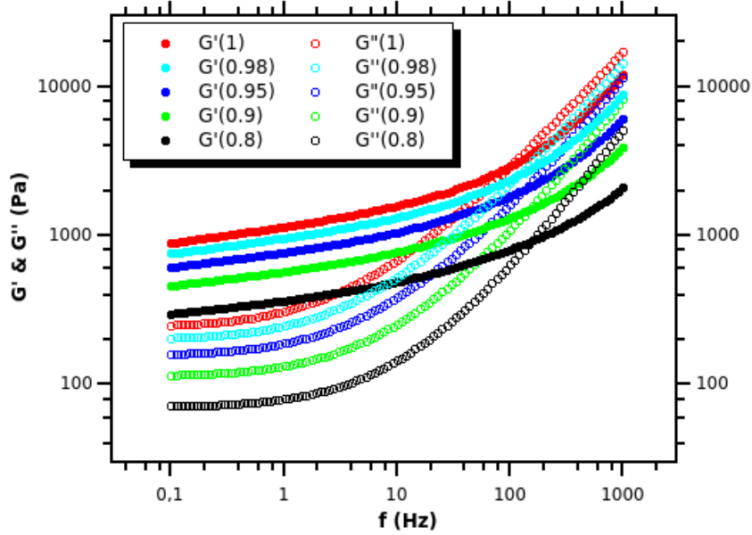
Figure 5: Predictions of the two-phase emulsion model for various cell concentrations \phi = 0.8, 0.9, 0.95, 0.98, 1 , \alpha/R=10^3 Pa, at collagen content c = 2 mg/mL.
