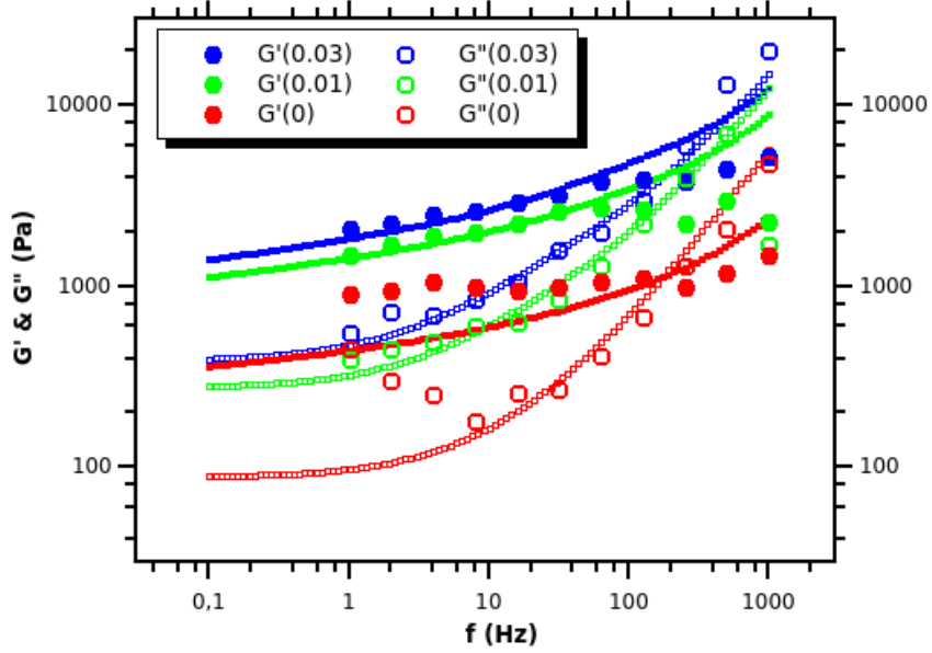
Figure 7: Spheroid properties ( G' , filled circles, and G'' , empty circles) for three initial collagen contents c_0 = 0 \text{ mg/mL} , 0.01 \text{ mg/mL} and 0.03 \text{ mg/mL} (19). Fits were made using the two-phase model with the respective optimal parameters ( c=2 \text{ mg/mL} , \phi=0.82 , \alpha/R=30 \text{ mN/m} ), ( c=4 \text{ mg/mL} , \phi=0.88 , \alpha/R=60 \text{ mN/m} ) and ( c=4 \text{ mg/mL} , \phi=0.94 , \alpha/R=80 \text{ mN/m} ).
