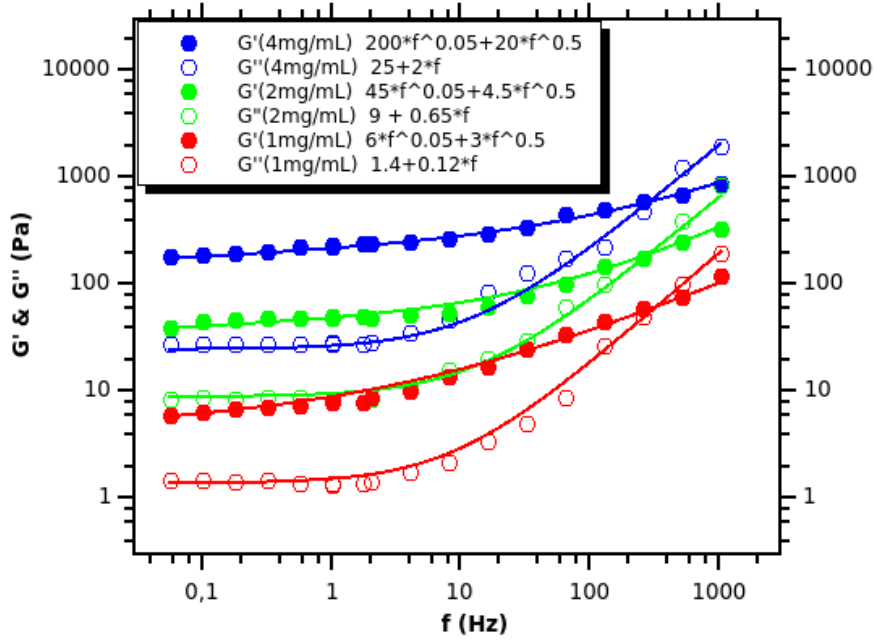
Figure 1: Rheological properties of the collagen matrix for three concentrations ( c = 1\text{mg/mL} , 2\text{ mg/mL} and 4\text{mg/mL} ). Data are collected from classical rheology [0.05Hz-10Hz] and AFM rheology [1Hz-1kHz].
