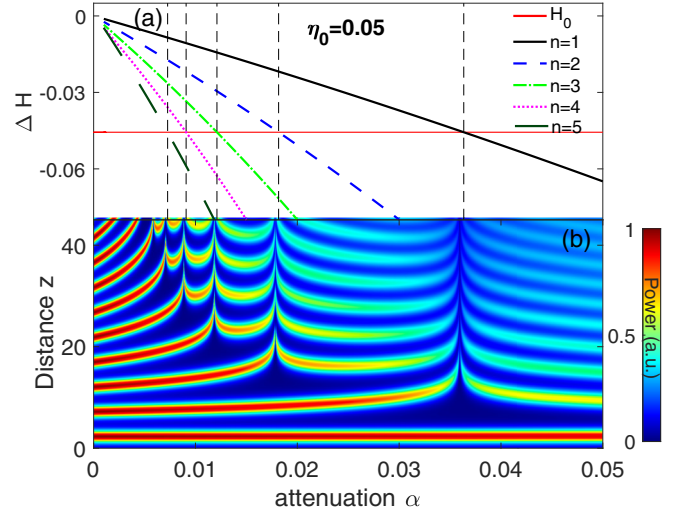
FIG. 8. (a) Variation of the Hamiltonian \Delta H(\alpha) vs attenuation \alpha , for n = 1, 2, 3, 4, 5 passages in the unshifted orbit. Vertical dashed lines mark the critical damping values \alpha = \alpha_{cn} , given by crossing of \Delta H(\alpha) with -H_0 (red horizontal line). (b) False color plot of sidebands power fraction \eta(z) vs \alpha obtained from numerical integration of Eqs. (A3) and (A4). Here \omega = \sqrt{2} and \eta_0 = 0.05 , as in Fig. 1 of the paper.
