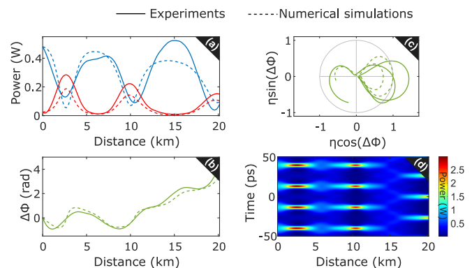
FIG. 6. Same as in Fig. 5. Experimental data are obtained with P_R = 170 mW, numerical simulations with \alpha_{\text{eff}} = 0.09 dB/km (region 2).
