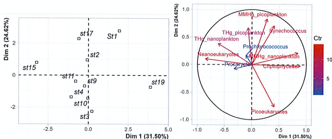
1146 1147 Figure S1: Principal component analysis of the phytoplankton composition ( Synechococcus spp., 1148 Prochlorococcus spp., picoeukaryotes, nanoeukaryotes and cryptophyceae), THg and MMHg in the 0.7–2.7 and 1149 2.7–20 \mu\text{m} size-fractions by station. Color gradient indicates the contribution of the variables from blue for low 1150 contribution to red for high contribution.
