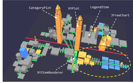
(a) JFreeChart, usage level 2, orientation OUT, JFreeChart and Plot as entry points. Displaying links of Plot reveals that XYPlot and CategoryPlot are subclasses. (b) Figure 7a after adding XYPlot and CategoryPlot as entry points
