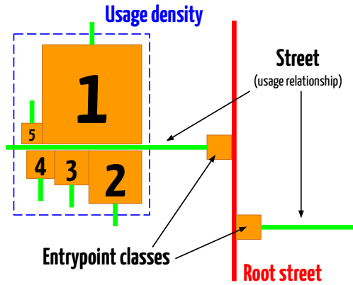
Figure 3: Placement algorithm
