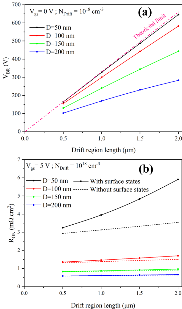
FIGURE 8. Evolution of breakdown voltage V_{BR} (a) and on-state resistance R_{ON} (b) as a function of drift region length for several nanowire diameters, with and without surface states.
