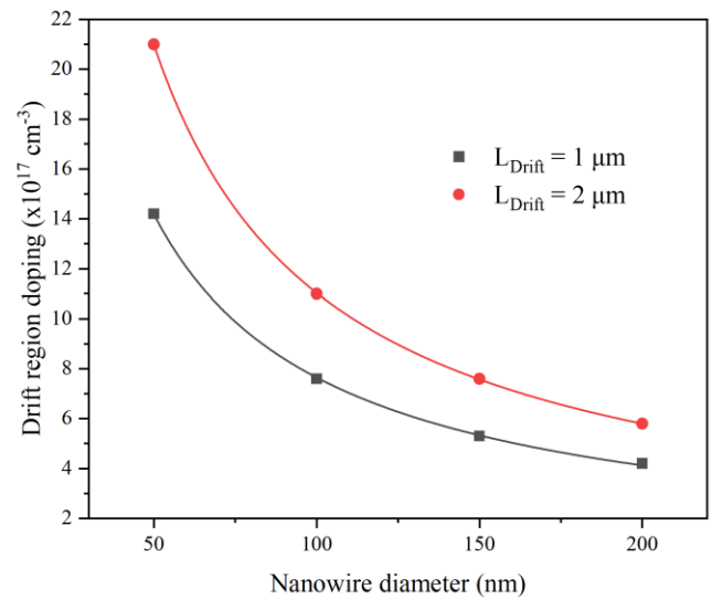
FIGURE 11. Best doping level to achieve a good R_{ON} as a function of the nanowire diameter for two different lengths of the drift region.
