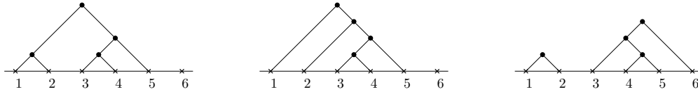
Figure 6: Shapes of equivalence classes for \text{Red}(21543)
