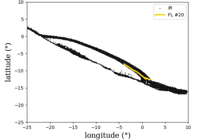
Fig. 7. Longitudinal-latitude connectivity map at 5 R_\odot displaying locations impacted by reconnection at the pseudo-streamer. The magnetic field lines connected to the black point in the figures have experienced at least one episode of magnetic reconnection during the course of the simulation. The yellow line traces the path of the intersection with the 5 R_\odot sphere of the magnetic field line n^{\circ}20 , as it slip-reconnects (see Sect. 3.7).
