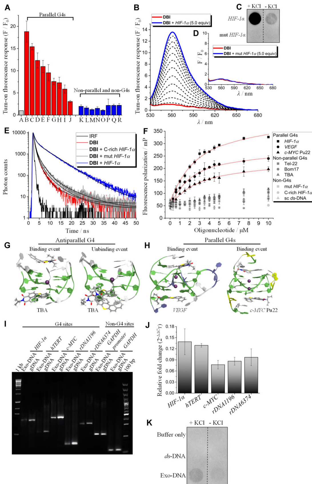
Figure 4. DBI binds to G4 structures. (A) DBI-associated turn-on fluorescence response upon individual addition of DNA structures. DBI (1 \mu M , DMSO 0.1% v/v) and oligonucleotides (5 \mu M ) were mixed together in TRIS buffer (50 mM, pH 7.2) and KCl (100 mM) and allowed to equilibrate at 25°C for 30
